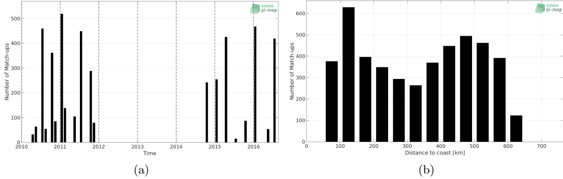
Figure 1: Number of match-ups between TSG-LEGOS-DM and SMOS L3 v2 - Monthly - 0.25 Deg (CATDS-CECOS-IFREMER) SSS as a function of time (a) and as function of the distance to coast (b) over the Ganga and Brahmaputra river plumes Pi-MEP region and for the full satellite product period.
