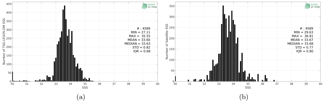
Figure 2: Histograms of SSS from TSG-LEGOS-DM (a) and SMOS L3 v2 - Monthly - 0.25 Deg (CATDS-CECOS-IFREMER) (b) considering all match-up pairs per bins of 0.1 over the Ganga and Brahmaputra river plumes Pi-MEP region and for the full satellite product period.
