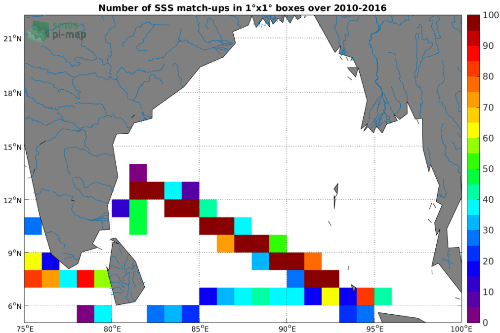
Figure 4: Number of SSS match-ups between TSG-LEGOS-DM SSS and the SMOS L3 v2 - Monthly - 0.25 Deg (CATDS-CECOS-IFREMER) SSS product for the Ganga and Brahmaputra river plumes Pi-MEP region over 1°x1° boxes and for the full satellite product period.
