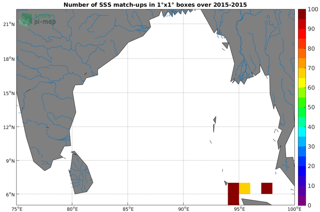
Figure 4: Number of SSS match-ups between TSG (SAMOS) SSS and the SMOS SSS L3 v2 - Daily - 0.5 Deg (CATDS-CECOS-IFREMER) SSS product for the Ganga and Brahmaputra river plumes Pi-MEP region over 1°x1° boxes and for the full satellite product period.
