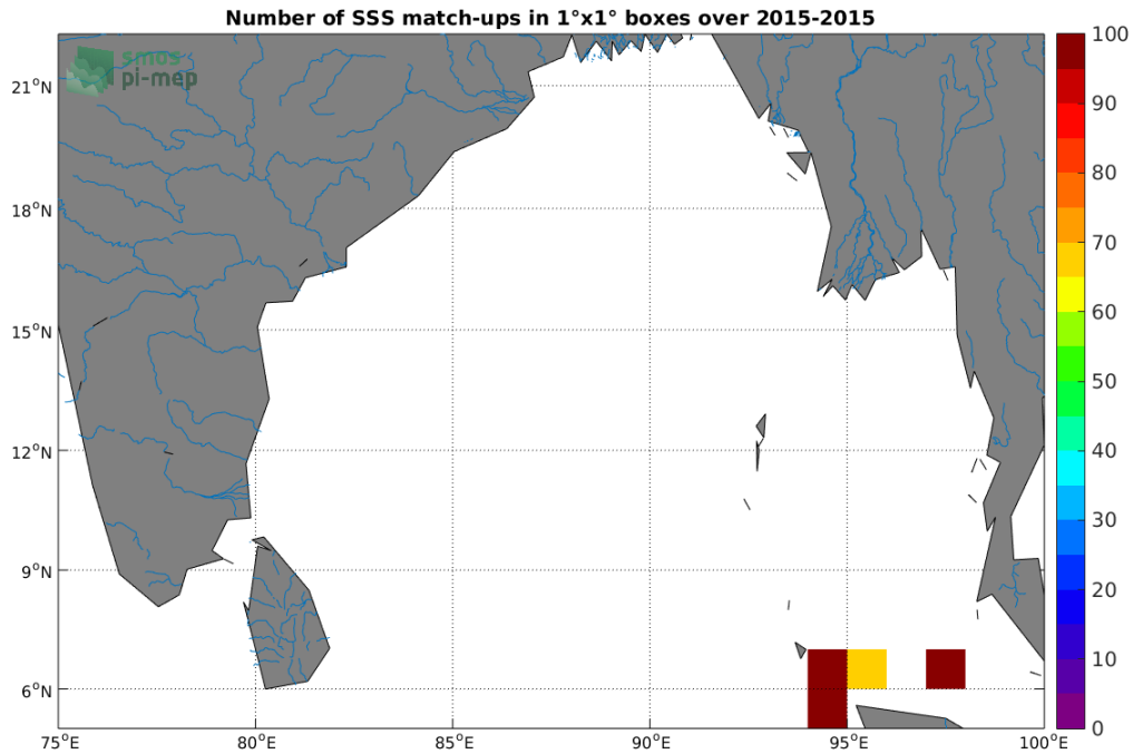
Figure 4: Number of SSS match-ups between TSG-SAMOS SSS and the SMOS L3 v2 - Daily - 0.5 Deg (CATDS-CECOS-IFREMER) SSS product for the Ganga and Brahmaputra river plumes Pi-MEP region over 1°x1° boxes and for the full satellite product period.
