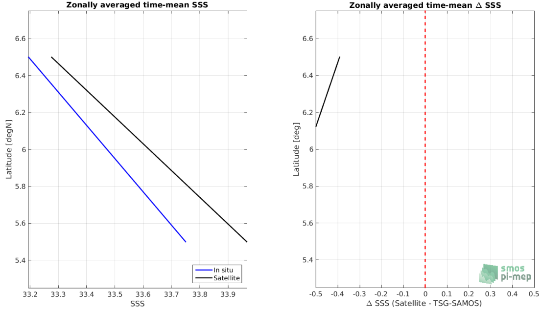
Figure 8: Left panel: Zonal mean SSS from SMOS L3 v2 - Daily - 0.5 Deg (CATDS-CECOS-IFREMER) satellite product (black) and from TSG-SAMOS (blue). Right panel: Zonal mean of \Delta SSS (Satellite - TSG-SAMOS) for all the collected Pi-MEP match-up pairs estimated over the full satellite product period.
