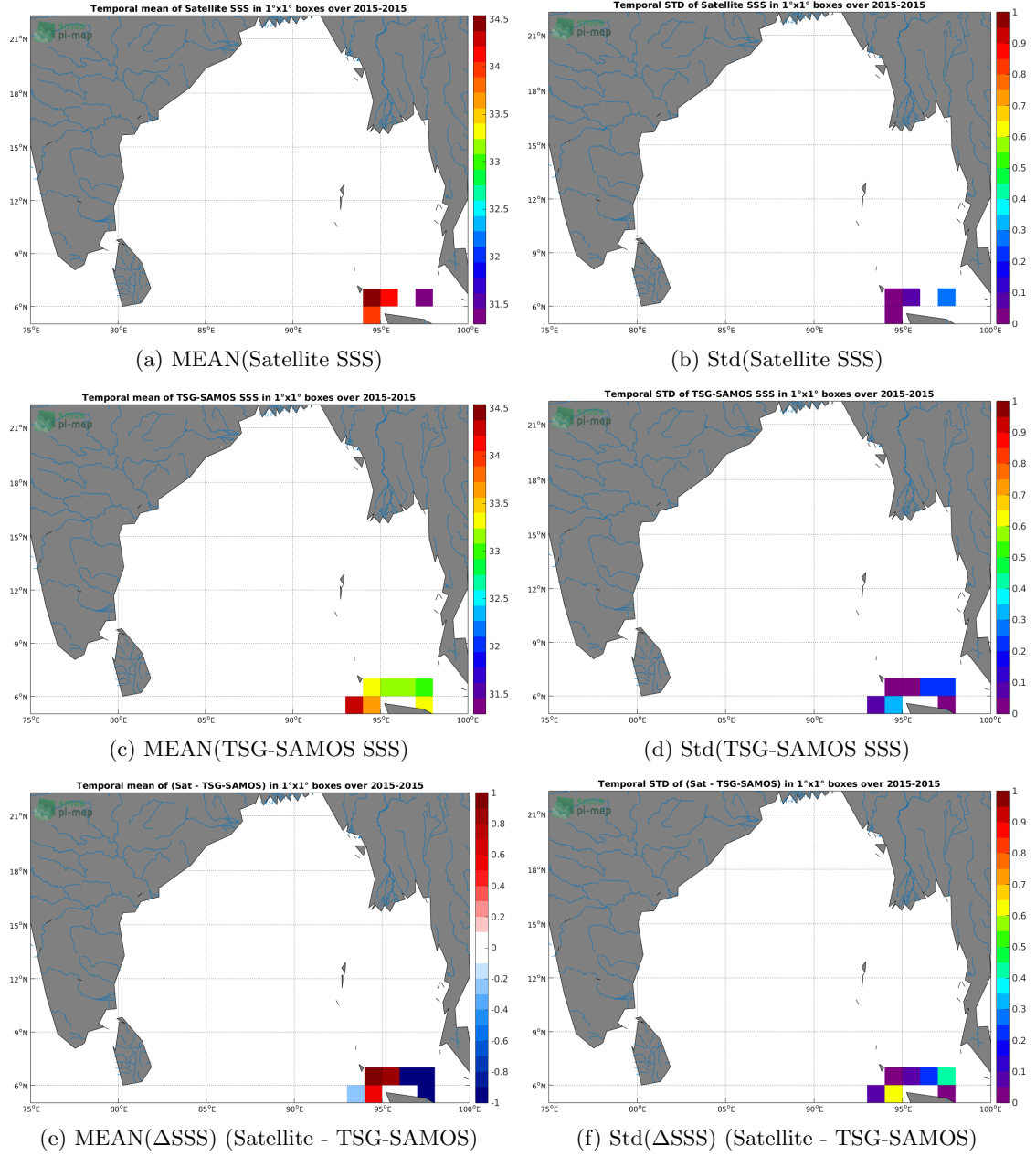
Figure 6: Temporal mean (left) and Std (right) of SSS from SMOS L3 v2 - Daily - 0.5 Deg (CATDS-CECOS-IFREMER) (top), TSG-SAMOS (middle), and of \Delta SSS (Satellite - TSG-SAMOS). Only match-up pairs are used to generate these maps.
