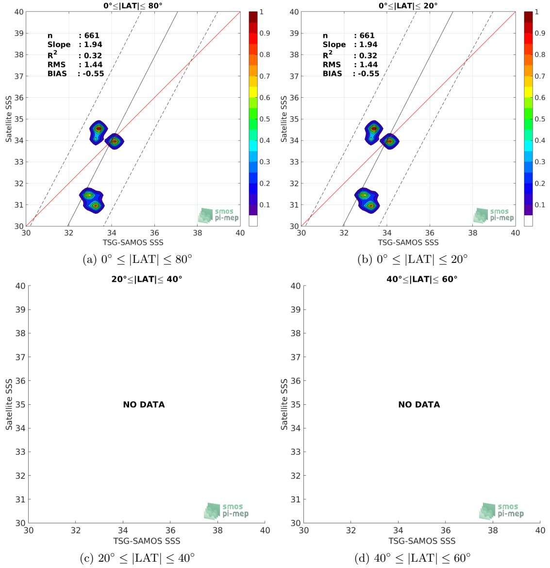
Figure 9: Contour maps of the concentration of SMOS L3 v2 - Daily - 0.5 Deg (CATDS-CECOS-IFREMER) SSS (y-axis) versus TSG-SAMOS SSS (x-axis) at match-up pairs for different latitude bands. For each plot, the red line shows x=y . The black thin and dashed lines indicate a linear fit through the data cloud and the \pm 95\% confidence levels, respectively. The number match-up pairs n , the slope and R^2 coefficient of the linear fit, the root mean square (RMS) and the mean bias between satellite and in situ data are indicated for each latitude band in each plots.
