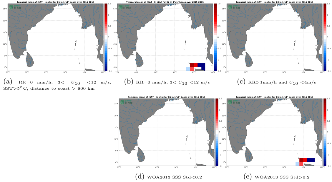
Figure 12: Temporal mean gridded over spatial boxes of size 1^\circ \times 1^\circ of \Delta SSS (SMOS L3 v2 - Daily - 0.5 Deg (CATDS-CECOS-IFREMER) - TSG-SAMOS) for 5 different subdatasets corresponding to: RR=0 mm/h, 3 < U_{10} < 12 m/s, SST > 5^\circ C , distance to coast > 800 km (a), RR=0 mm/h, 3 < U_{10} < 12 m/s (b), RR > 1 mm/h and U_{10} < 4 m/s (c), WOA2013 SSS Std < 0.2 (d), WOA2013 SSS Std > 0.2 (e).
