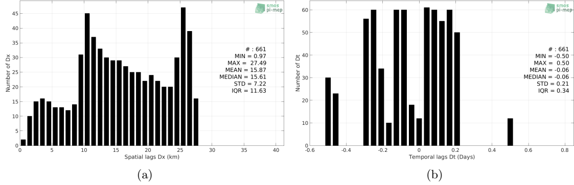
Figure 5: Histograms of the spatial (a) and temporal (b) lags between the time of the TSG-SAMOS measurements and the date of the corresponding SMOS L3 v2 - Daily - 0.5 Deg (CATDS-CECOS-IFREMER) SSS product.
