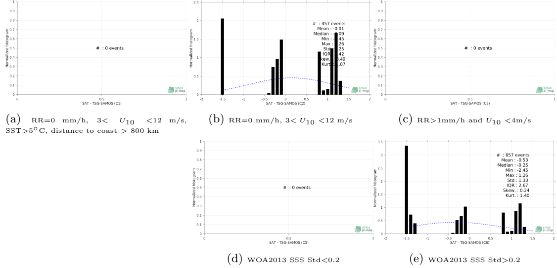
Figure 13: Normalized histogram of \Delta SSS (SMOS L3 v2 - Daily - 0.5 Deg (CATDS-CECOS-IFREMER) - TSG-SAMOS) for 5 different subdatasets corresponding to: RR=0 mm/h, 3 < U_{10} < 12 m/s, SST>5°C, distance to coast > 800 km (a), RR=0 mm/h, 3 < U_{10} < 12 m/s (b), RR>1mm/h and U_{10} < 4 m/s (c), WOA2013 SSS Std<0.2 (d), WOA2013 SSS Std>0.2 (e).
