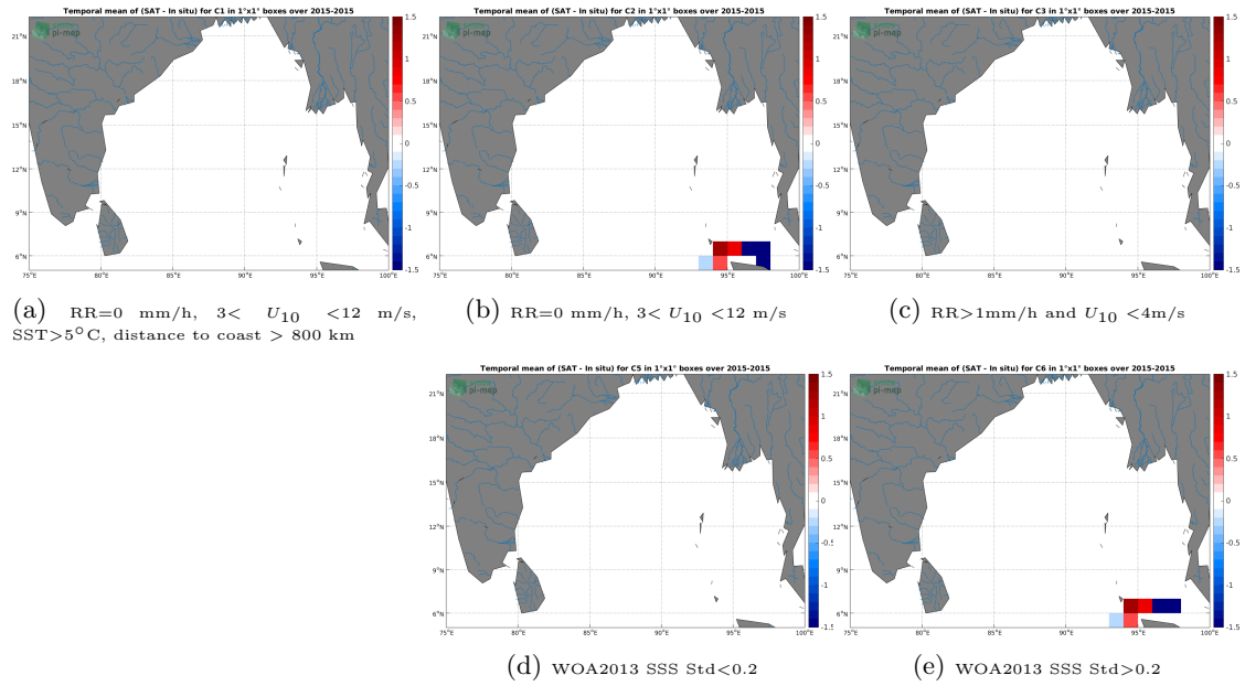
Figure 12: Temporal mean gridded over spatial boxes of size 1^\circ \times 1^\circ of \Delta SSS (SMOS-L3-CATDS-CECOS-IFREMER-V2-1DAY-0.5DEG - TSG-SAMOS) for 5 different subdatasets corresponding to: RR=0 mm/h, 3 < U_{10} < 12 m/s, SST > 5^\circ C , distance to coast > 800 km (a), RR=0 mm/h, 3 < U_{10} < 12 m/s (b), RR > 1 mm/h and U_{10} < 4 m/s (c), WOA2013 SSS Std < 0.2 (d), WOA2013 SSS Std > 0.2 (e).
