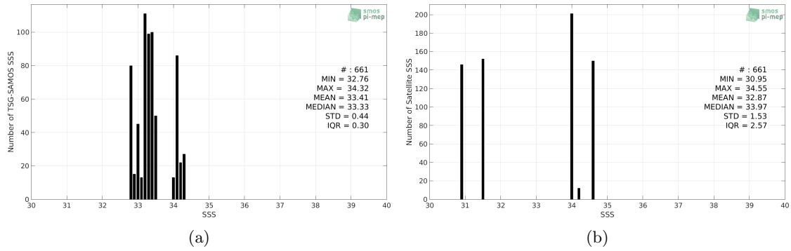
Figure 2: Histograms of SSS from TSG-SAMOS (a) and SMOS-L3-CATDS-CECOS-IFREMER-V2-1DAY-0.5DEG (b) considering all match-up pairs per bins of 0.1 over the Ganga and Brahmaputra river plumes Pi-MEP region and for the full satellite product period.
