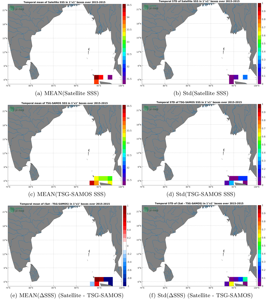
Figure 6: Temporal mean (left) and Std (right) of SSS from SMOS-L3-CATDS-CECOS-IFREMER-V2-1DAY-0.5DEG (top), TSG-SAMOS (middle), and of \Delta SSS (Satellite - TSG-SAMOS). Only match-up pairs are used to generate these maps.
