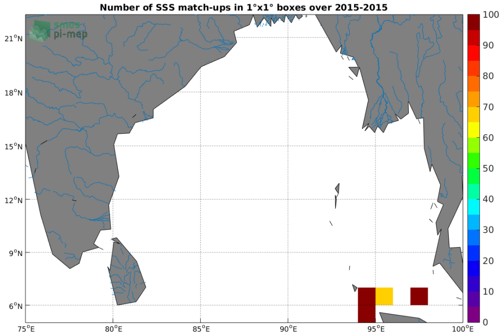
Figure 4: Number of SSS match-ups between TSG-SAMOS SSS and the SMOS-L3-CATDS-CECOS-IFREMER-V2-1DAY-0.5DEG SSS product for the Ganga and Brahmaputra river plumes Pi-MEP region over 1°x1° boxes and for the full satellite product period.
