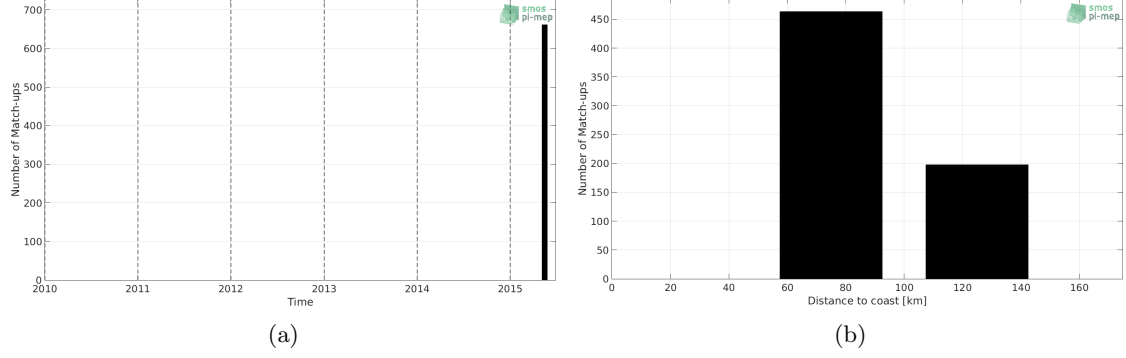
Figure 1: Number of match-ups between TSG-SAMOS and SMOS-L3-CATDS-CECOS-IFREMER-V2-1DAY-0.5DEG SSS as a function of time (a) and as function of the distance to coast (b) over the Ganga and Brahmaputra river plumes Pi-MEP region and for the full satellite product period.
