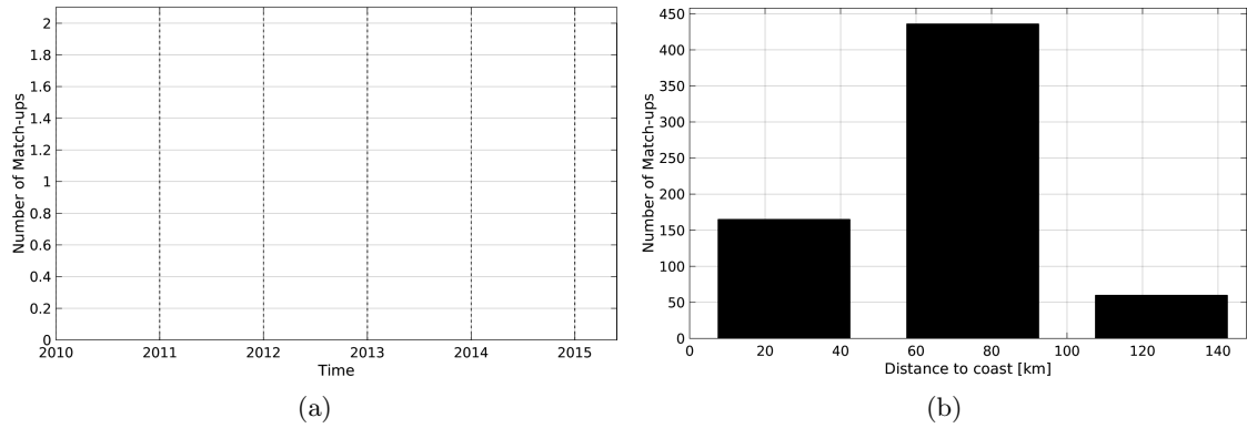
Figure 1: Number of match-ups between TSG-SAMOS and SMOS-L3-CATDS-CECOS-IFREMER-V2-1DAY-0.5deg SSS as a function of time (a) and as function of the distance to coast (b) over the Ganga and Brahmaputra river plumes Pi-MEP region and for the full satellite product period.
