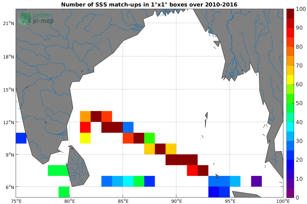
Figure 4: Number of SSS match-ups between TSG (LEGOS-DM) SSS and the SMOS SSS L3 v2 - Daily - 0.5 Deg (CATDS-CECOS-IFREMER) SSS product for the Ganga and Brahmaputra river plumes Pi-MEP region over 1°x1° boxes and for the full satellite product period.
