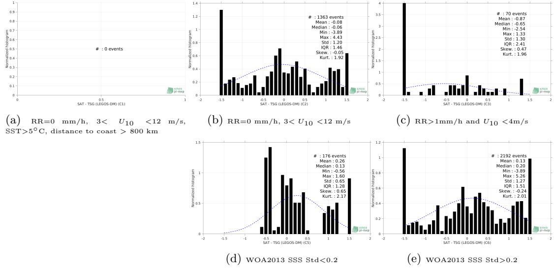
Figure 13: Normalized histogram of \Delta SSS (SMOS SSS L3 v2 - Daily - 0.5 Deg (CATDS-CECOS-IFREMER) - TSG (LEGOS-DM)) for 5 different subdatasets corresponding to: RR=0 mm/h, 3 < U_{10} < 12 m/s, SST>5°C, distance to coast > 800 km (a), RR=0 mm/h, 3 < U_{10} < 12 m/s (b), RR>1mm/h and U_{10} < 4 m/s (c), WOA2013 SSS Std<0.2 (d), WOA2013 SSS Std>0.2 (e).
