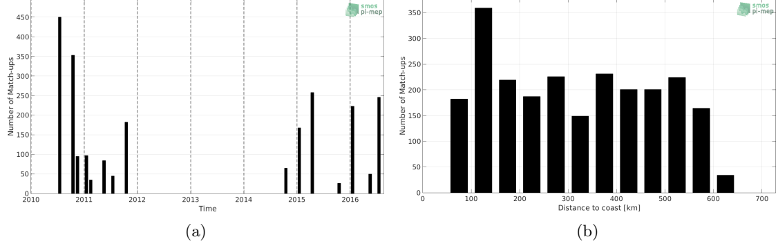
Figure 1: Number of match-ups between TSG (LEGOS-DM) and SMOS SSS L3 v2 - Daily - 0.5 Deg (CATDS-CECOS-IFREMER) SSS as a function of time (a) and as function of the distance to coast (b) over the Ganga and Brahmaputra river plumes Pi-MEP region and for the full satellite product period.
