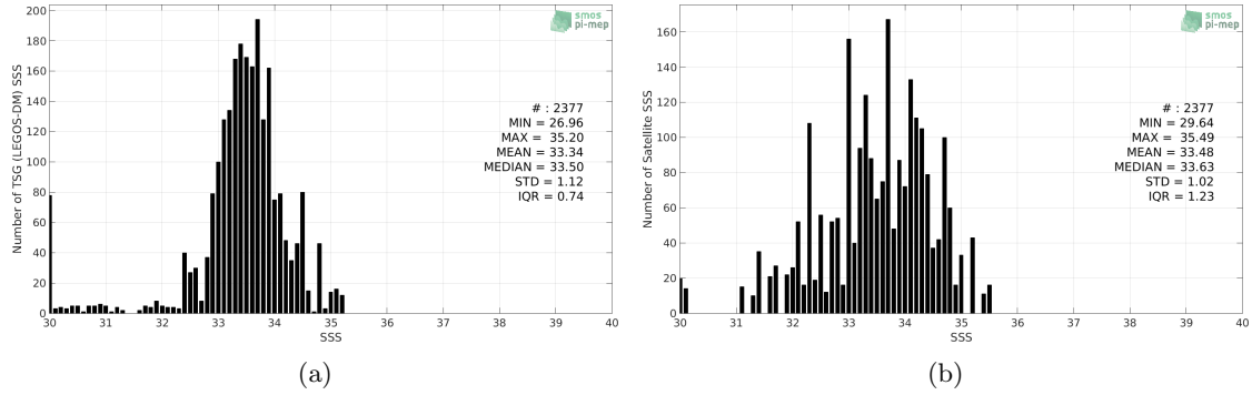
Figure 2: Histograms of SSS from TSG (LEGOS-DM) (a) and SMOS SSS L3 v2 - Daily - 0.5 Deg (CATDS-CECOS-IFREMER) (b) considering all match-up pairs per bins of 0.1 over the Ganga and Brahmaputra river plumes Pi-MEP region and for the full satellite product period.
