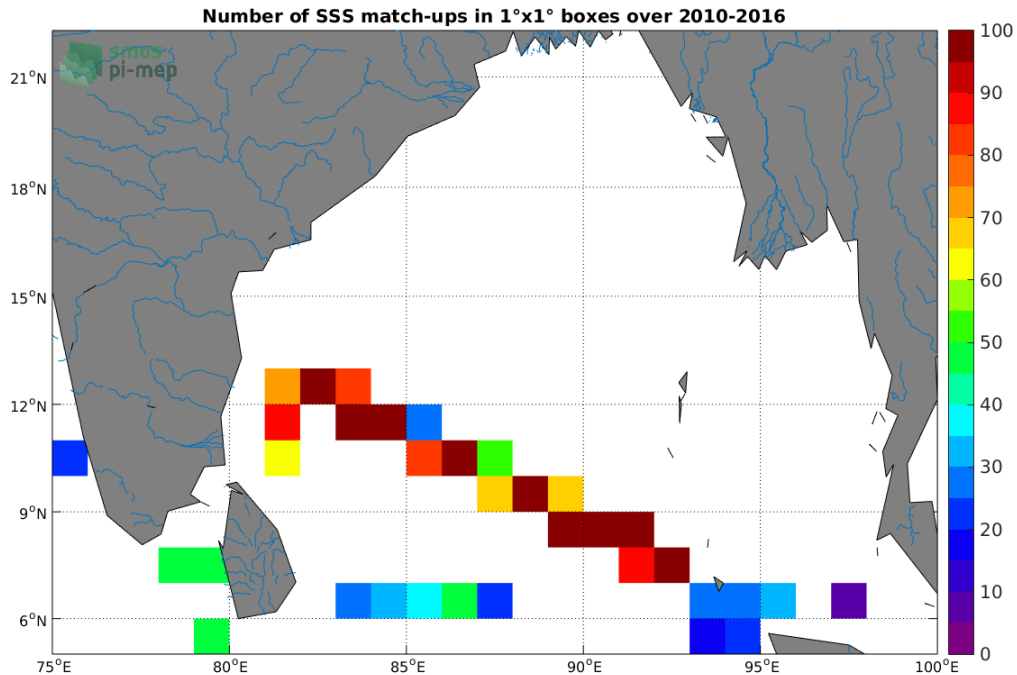
Figure 4: Number of SSS match-ups between TSG-LEGOS-DM SSS and the SMOS L3 v2 - Daily - 0.5 Deg (CATDS-CECOS-IFREMER) SSS product for the Ganga and Brahmaputra river plumes Pi-MEP region over 1°x1° boxes and for the full satellite product period.
