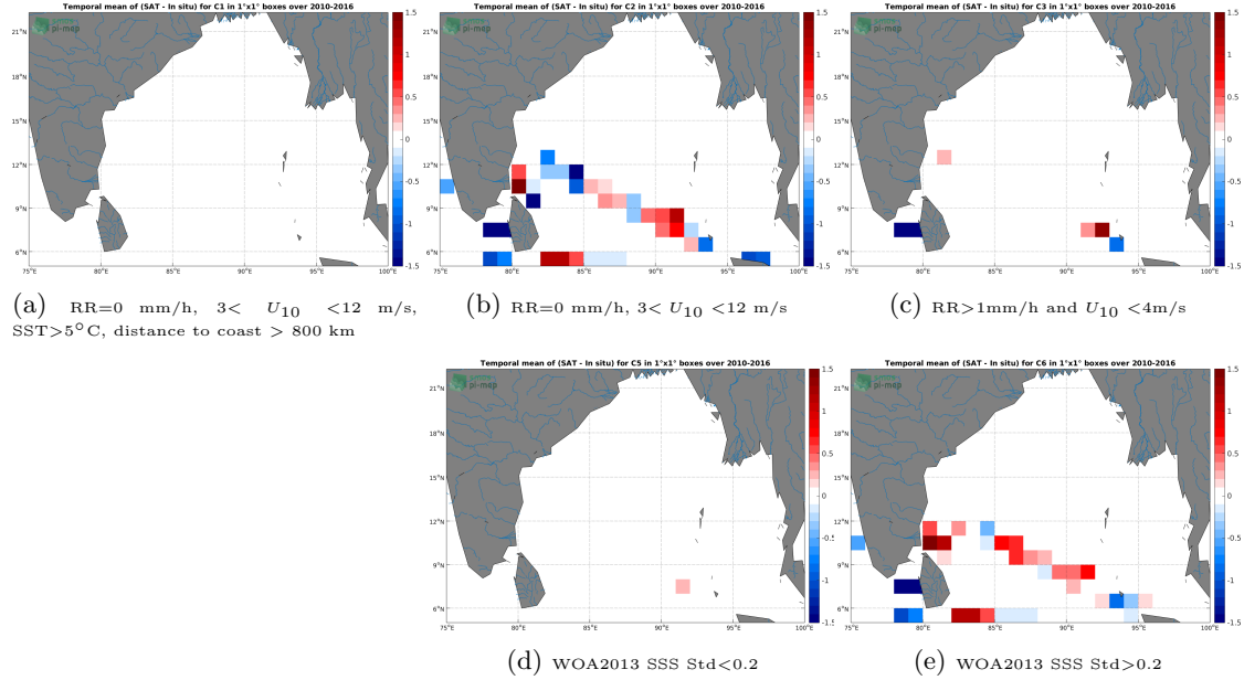
Figure 12: Temporal mean gridded over spatial boxes of size 1^{\circ}\times 1^{\circ} of \Delta\text{SSS} (SMOS L3 v2 - Daily - 0.5 Deg (CATDS-CECOS-IFREMER) - TSG-LEGOS-DM) for 5 different subdatasets corresponding to: RR=0 mm/h, 3 < U_{10} < 12 m/s, SST >5^{\circ}\text{C} , distance to coast > 800 km (a), RR=0 mm/h, 3 < U_{10} < 12 m/s (b), RR >1 mm/h and U_{10} < 4 m/s (c), WOA2013 SSS Std <0.2 (d), WOA2013 SSS Std >0.2 (e).
