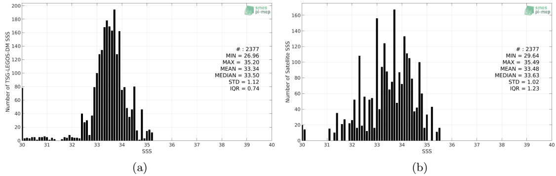
Figure 2: Histograms of SSS from TSG-LEGOS-DM (a) and SMOS L3 v2 - Daily - 0.5 Deg (CATDS-CECOS-IFREMER) (b) considering all match-up pairs per bins of 0.1 over the Ganga and Brahmaputra river plumes Pi-MEP region and for the full satellite product period.
