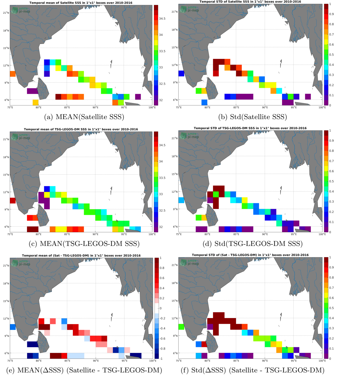
Figure 6: Temporal mean (left) and Std (right) of SSS from SMOS L3 v2 - Daily - 0.5 Deg (CATDS-CECOS-IFREMER) (top), TSG-LEGOS-DM (middle), and of \Delta SSS (Satellite - TSG-LEGOS-DM). Only match-up pairs are used to generate these maps.
