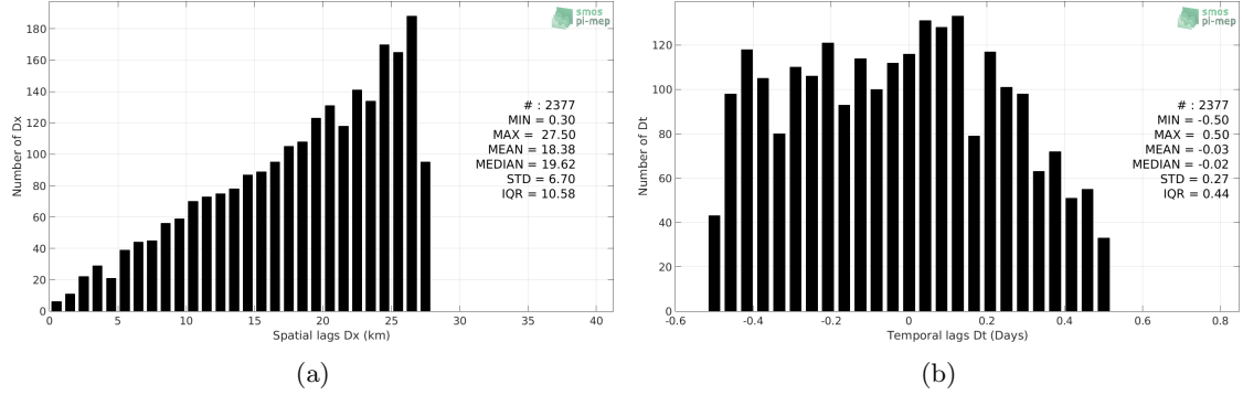
Figure 5: Histograms of the spatial (a) and temporal (b) lags between the time of the TSG-LEGOS-DM measurements and the date of the corresponding SMOS L3 v2 - Daily - 0.5 Deg (CATDS-CECOS-IFREMER) SSS product.
