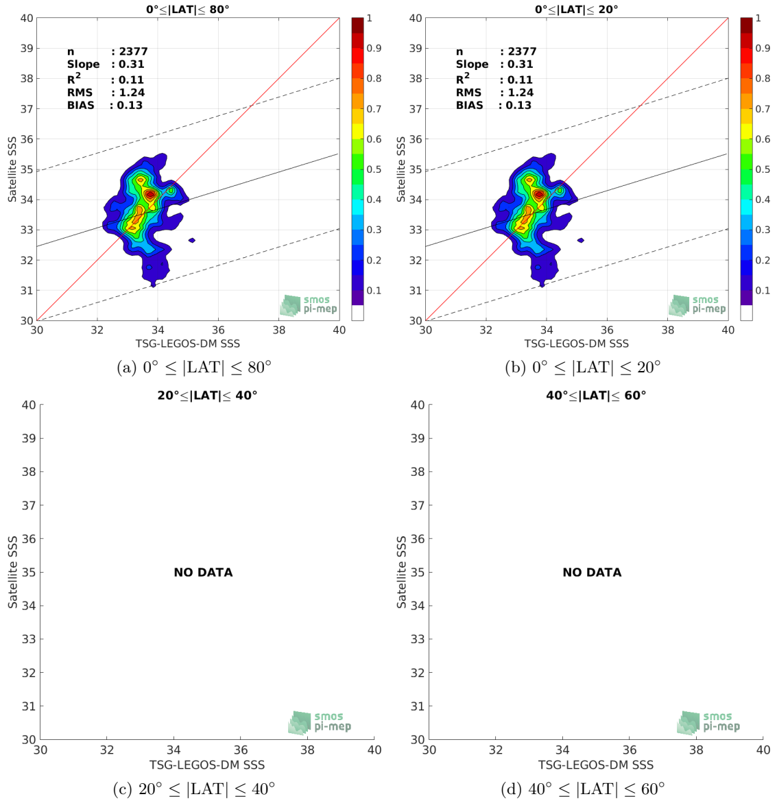
Figure 9: Contour maps of the concentration of SMOS L3 v2 - Daily - 0.5 Deg (CATDS-CECOS-IFREMER) SSS (y-axis) versus TSG-LEGOS-DM SSS (x-axis) at match-up pairs for different latitude bands. For each plot, the red line shows x=y . The black thin and dashed lines indicate a linear fit through the data cloud and the \pm 95\% confidence levels, respectively. The number match-up pairs n , the slope and R^2 coefficient of the linear fit, the root mean square (RMS) and the mean bias between satellite and in situ data are indicated for each latitude band in each plots.
