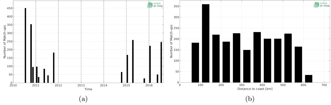
Figure 1: Number of match-ups between TSG-LEGOS-DM and SMOS L3 v2 - Daily - 0.5 Deg (CATDS-CECOS-IFREMER) SSS as a function of time (a) and as function of the distance to coast (b) over the Ganga and Brahmaputra river plumes Pi-MEP region and for the full satellite product period.
