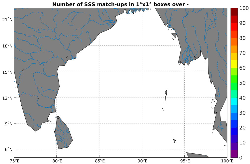
Figure 4: Number of SSS match-ups between TSG-GOSUD-Sailing-ship SSS and the SMOS-L3-CATDS-CECOS-IFREMER-V2-1DAY-0.5deg SSS product for the Ganga and Brahmaputra river plumes Pi-MEP region over 1°x1° boxes and for the full satellite product period.
