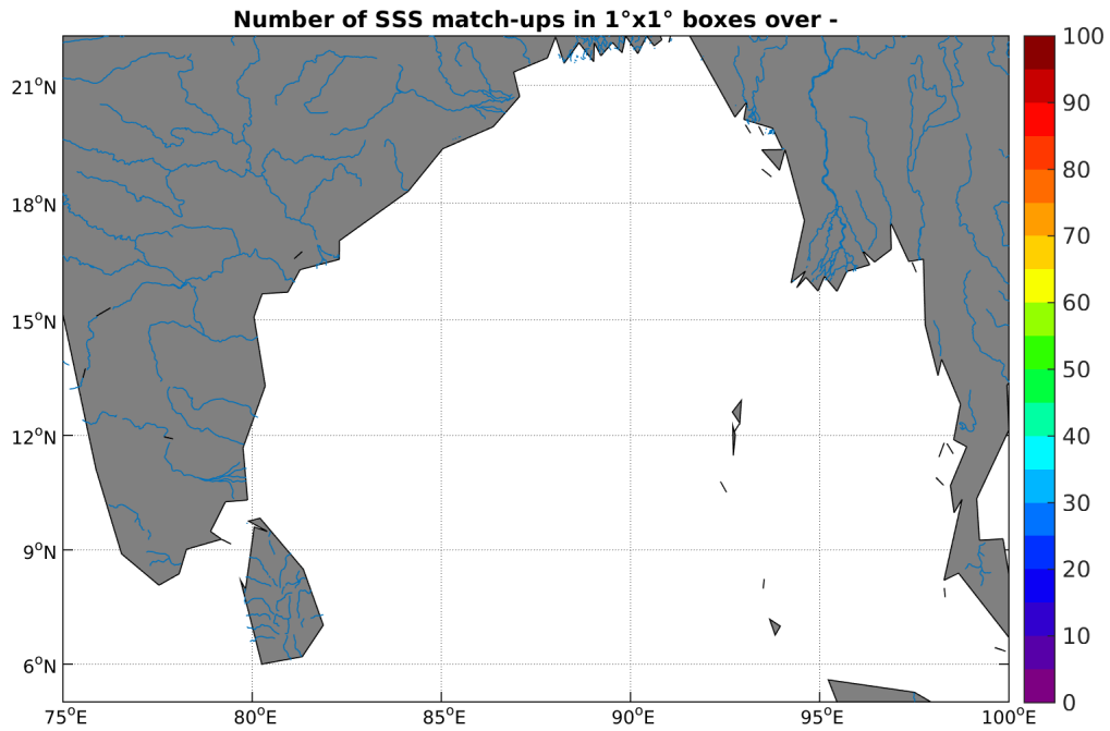
Figure 4: Number of SSS match-ups between TSG-GOSUD-Research-vessel SSS and the SMOS-L3-CATDS-CECOS-IFREMER-V2-1DAY-0.5deg SSS product for the Ganga and Brahmaputra river plumes Pi-MEP region over 1°x1° boxes and for the full satellite product period.
