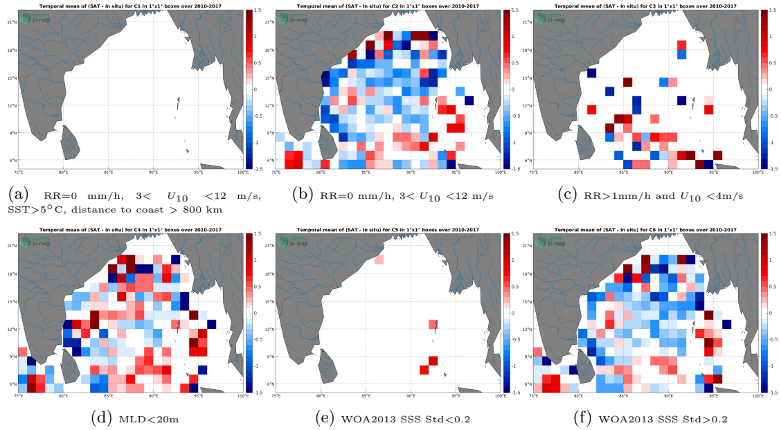
Figure 12: Temporal mean gridded over spatial boxes of size 1^\circ \times 1^\circ of \Delta SSS (SMOS L3 v2 - Daily - 0.5 Deg (CATDS-CECOS-IFREMER) - Argo) for 6 different subdatasets corresponding to: RR=0 mm/h, 3 < U_{10} < 12 m/s, SST >5^\circ C, distance to coast > 800 km (a), RR=0 mm/h, 3 < U_{10} < 12 m/s (b), RR >1 mm/h and U_{10} < 4 m/s (c),MLD <20 m (d),WOA2013 SSS Std <0.2 (e),WOA2013 SSS Std >0.2 (f).
