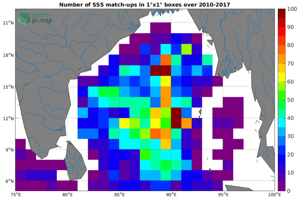
Figure 4: Number of SSS match-ups between Argo SSS and the SMOS L3 v2 - Daily - 0.5 Deg (CATDS-CECOS-IFREMER) SSS product for the Ganga and Brahmaputra river plumes Pi-MEP region over 1°x1° boxes and for the full satellite product period.
