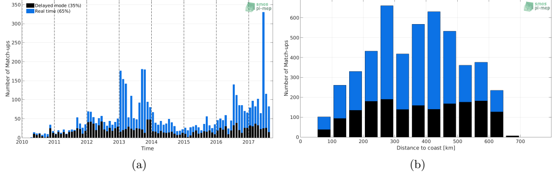
Figure 1: Number of match-ups between Argo and SMOS L3 v2 - Daily - 0.5 Deg (CATDS-CECOS-IFREMER) SSS as a function of time (a) and as function of the distance to coast (b) over the Ganga and Brahmaputra river plumes Pi-MEP region and for the full satellite product period.
