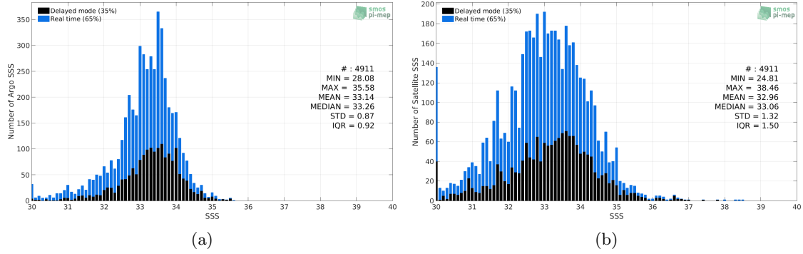
Figure 2: Histograms of SSS from Argo (a) and SMOS L3 v2 - Daily - 0.5 Deg (CATDS-CECOS-IFREMER) (b) considering all match-up pairs per bins of 0.1 over the Ganga and Brahmaputra river plumes Pi-MEP region and for the full satellite product period.
