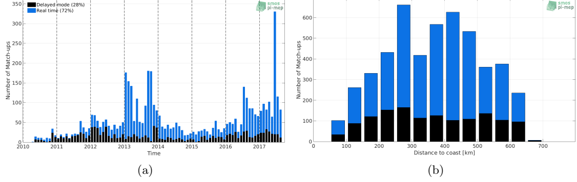
Figure 1: Number of match-ups between Argo and SMOS-L3-CATDS-CECOS-IFREMER-V2-1DAY-0.5DEG SSS as a function of time (a) and as function of the distance to coast (b) over the Ganga and Brahmaputra river plumes Pi-MEP region and for the full satellite product period.
