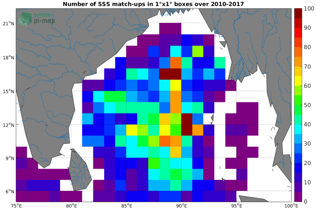
Figure 4: Number of SSS match-ups between Argos SSS and the SMOS-L3-CATDS-CECOS-IFREMER-V2-1DAY-0.5DEG SSS product for the Ganga and Brahmaputra river plumes Pi-MEP region over 1°x1° boxes and for the full satellite product period.
