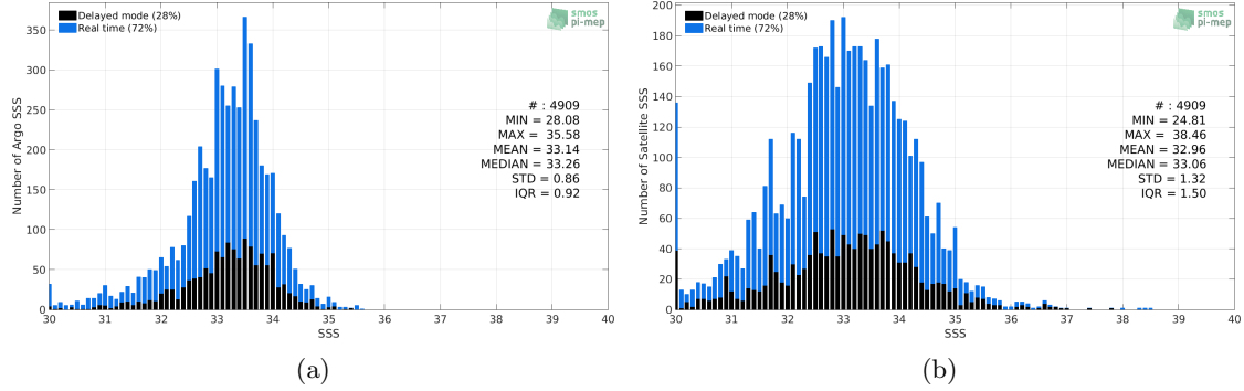
Figure 2: Histograms of SSS from Argo (a) and SMOS-L3-CATDS-CECOS-IFREMER-V2-1DAY-0.5DEG (b) considering all match-up pairs per bins of 0.1 over the Ganga and Brahmaputra river plumes Pi-MEP region and for the full satellite product period.
