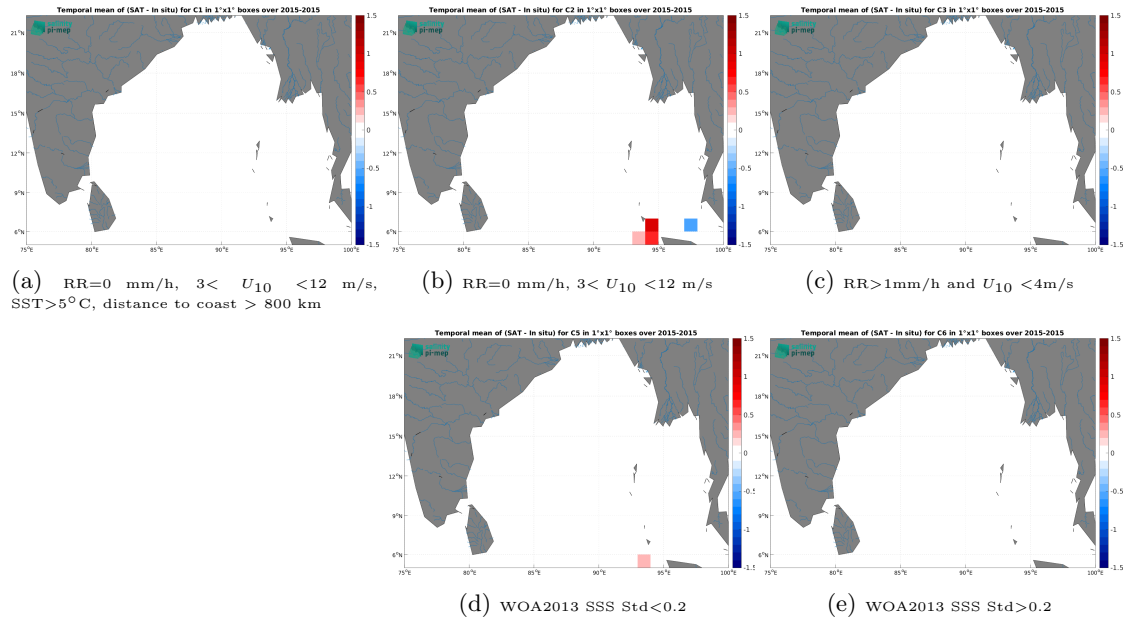
Figure 14: Temporal mean gridded over spatial boxes of size 1^\circ \times 1^\circ of \Delta SSS (SMOS SSS L3 v335 - Monthly - 25 km (CATDS-CPDC) - TSG (SAMOS)) for 5 different subdatasets corresponding to:RR=0 mm/h, 3 < U_{10} < 12 m/s, SST >5^\circ\text{C} , distance to coast > 800 km (a), RR=0 mm/h, 3 < U_{10} < 12 m/s (b), RR >1 mm/h and U_{10} < 4 m/s (c), WOA2013 SSS Std <0.2 (d), WOA2013 SSS Std >0.2 (e).
