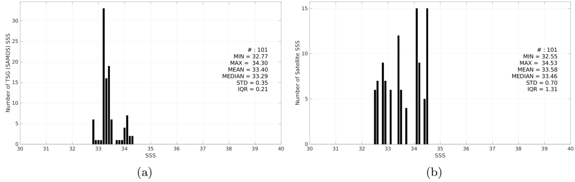
Figure 3: Histograms of SSS from TSG (SAMOS) (a) and SMOS SSS L3 v335 - Monthly - 25 km (CATDS-CPDC) (b) considering all match-up pairs per bins of 0.1 over the Ganga and Brahmaputra river plumes Pi-MEP region and for the full satellite product period.
