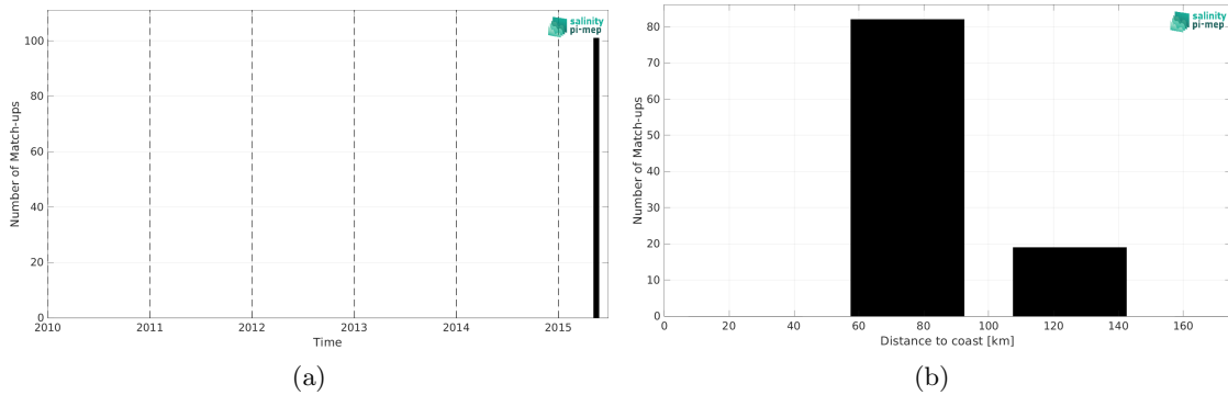
Figure 2: Number of match-ups between TSG (SAMOS) and SMOS SSS L3 v335 - Monthly - 25 km (CATDS-CPDC) SSS as a function of time (a) and as function of the distance to coast (b) over the Ganga and Brahmaputra river plumes Pi-MEP region and for the full satellite product period.
