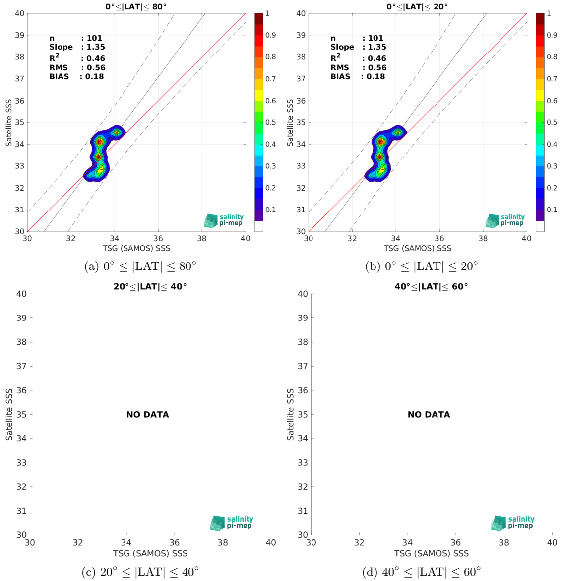
Figure 10: Contour maps of the concentration of SMOS SSS L3 v335 - Monthly - 25 km (CATDS-CPDC) SSS (y-axis) versus TSG (SAMOS) SSS (x-axis) at match-up pairs for different latitude bands. For each plot, the red line shows x=y . The black thin and dashed lines indicate a linear fit through the data cloud and the \pm 95\% confidence levels, respectively. The number match-up pairs n , the slope and R^2 coefficient of the linear fit, the root mean square (RMS) and the mean bias between satellite and in situ data are indicated for each latitude band in each plots.
