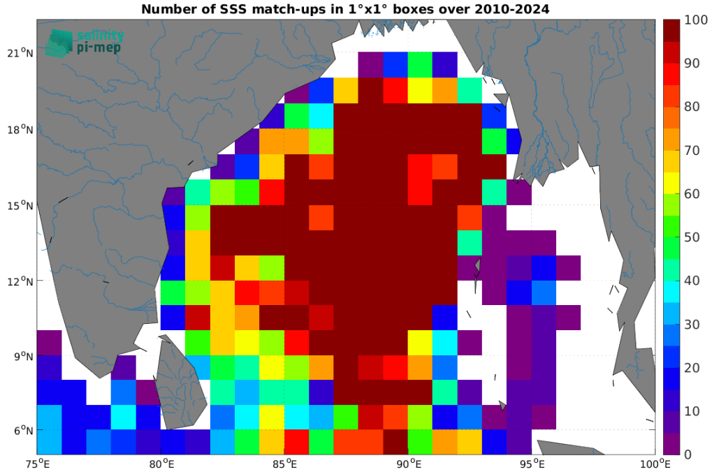
Figure 5: Number of SSS match-ups between Argo SSS and the SMOS SSS L3 v335 - Monthly - 25 km (CATDS-CPDC) SSS product for the Ganga and Brahmaputra river plumes Pi-MEP region over 1^\circ \times 1^\circ boxes and for the full satellite product period.
