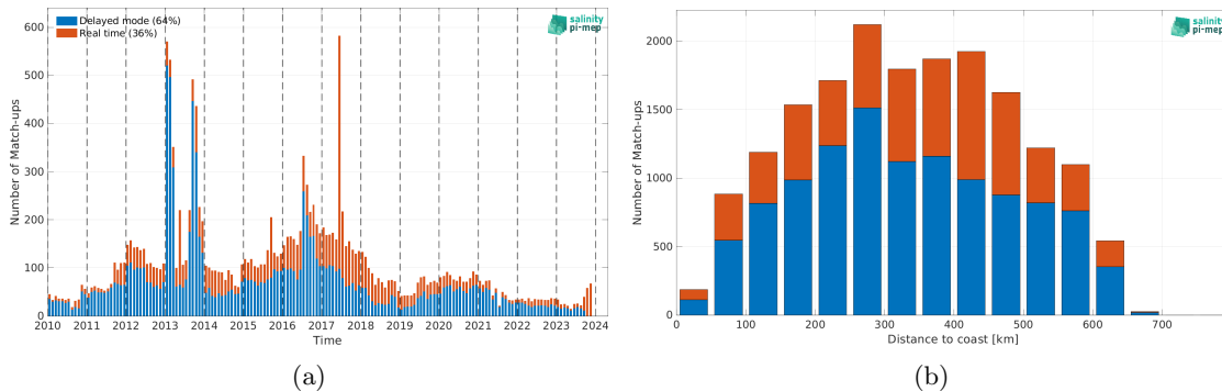
Figure 2: Number of match-ups between Argo and SMOS SSS L3 v335 - Monthly - 25 km (CATDS-CPDC) SSS as a function of time (a) and as function of the distance to coast (b) over the Ganga and Brahmaputra river plumes Pi-MEP region and for the full satellite product period.
