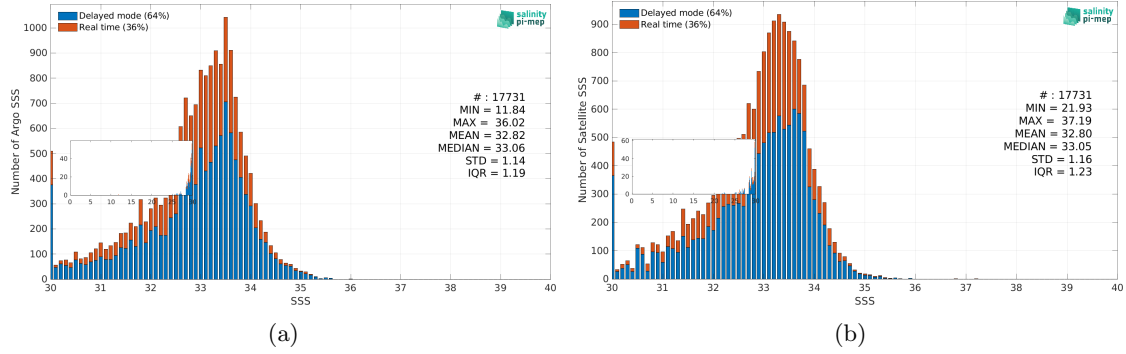
Figure 3: Histograms of SSS from Argo (a) and SMOS SSS L3 v335 - Monthly - 25 km (CATDS-CPDC) (b) considering all match-up pairs per bins of 0.1 over the Ganga and Brahmaputra river plumes Pi-MEP region and for the full satellite product period.
