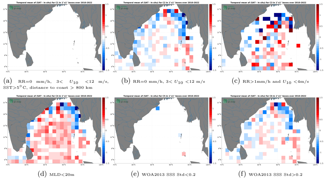
Figure 12: Temporal mean gridded over spatial boxes of size 1^\circ \times 1^\circ of \Delta SSS (SMOS SSS L3 v335 - Monthly - 25 km (CATDS-CPDC) - Argo) for 6 different subdatasets corresponding to: RR=0 mm/h, 3 < U_{10} < 12 m/s, SST > 5^\circ C , distance to coast > 800 km (a), RR=0 mm/h, 3 < U_{10} < 12 m/s (b), RR > 1 mm/h and U_{10} < 4 m/s (c), MLD < 20 m (d), WOA2013 SSS Std < 0.2 (e), WOA2013 SSS Std > 0.2 (f).
