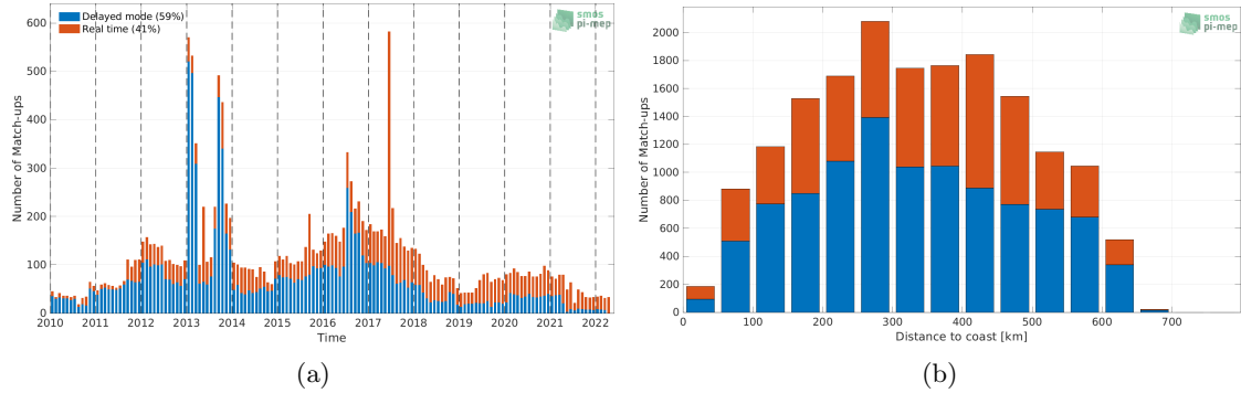
Figure 1: Number of match-ups between Argo and SMOS SSS L3 v335 - Monthly - 25 km (CATDS-CPDC) SSS as a function of time (a) and as function of the distance to coast (b) over the Ganga and Brahmaputra river plumes Pi-MEP region and for the full satellite product period.
