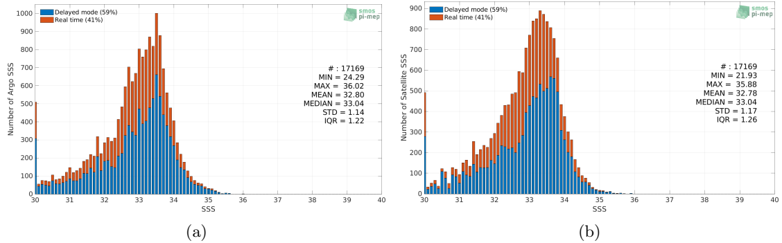
Figure 2: Histograms of SSS from Argo (a) and SMOS SSS L3 v335 - Monthly - 25 km (CATDS-CPDC) (b) considering all match-up pairs per bins of 0.1 over the Ganga and Brahmaputra river plumes Pi-MEP region and for the full satellite product period.
