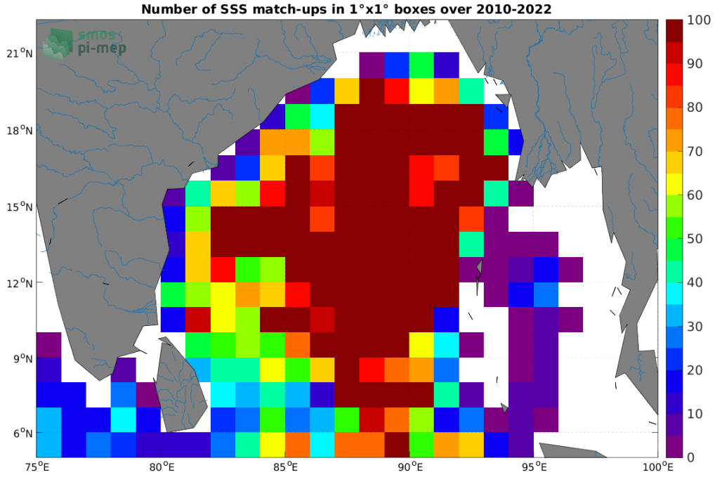
Figure 4: Number of SSS match-ups between Argo SSS and the SMOS SSS L3 v335 - Monthly - 25 km (CATDS-CPDC) SSS product for the Ganga and Brahmaputra river plumes Pi-MEP region over 1^\circ \times 1^\circ boxes and for the full satellite product period.
