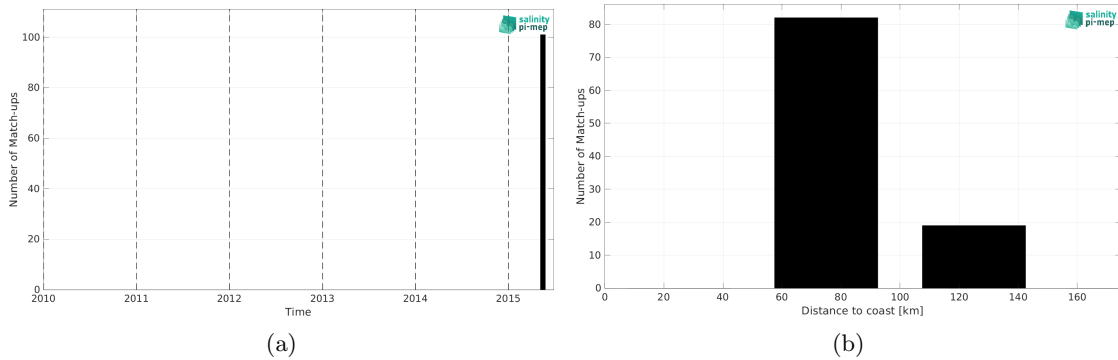
Figure 2: Number of match-ups between TSG (SAMOS) and SMOS SSS L3 v335 - 10 Days - 25 km (CATDS-CPDC) SSS as a function of time (a) and as function of the distance to coast (b) over the Ganga and Brahmaputra river plumes Pi-MEP region and for the full satellite product period.
