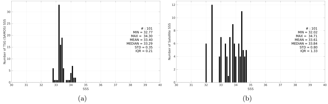
Figure 3: Histograms of SSS from TSG (SAMOS) (a) and SMOS SSS L3 v335 - 10 Days - 25 km (CATDS-CPDC) (b) considering all match-up pairs per bins of 0.1 over the Ganga and Brahmaputra river plumes Pi-MEP region and for the full satellite product period.
