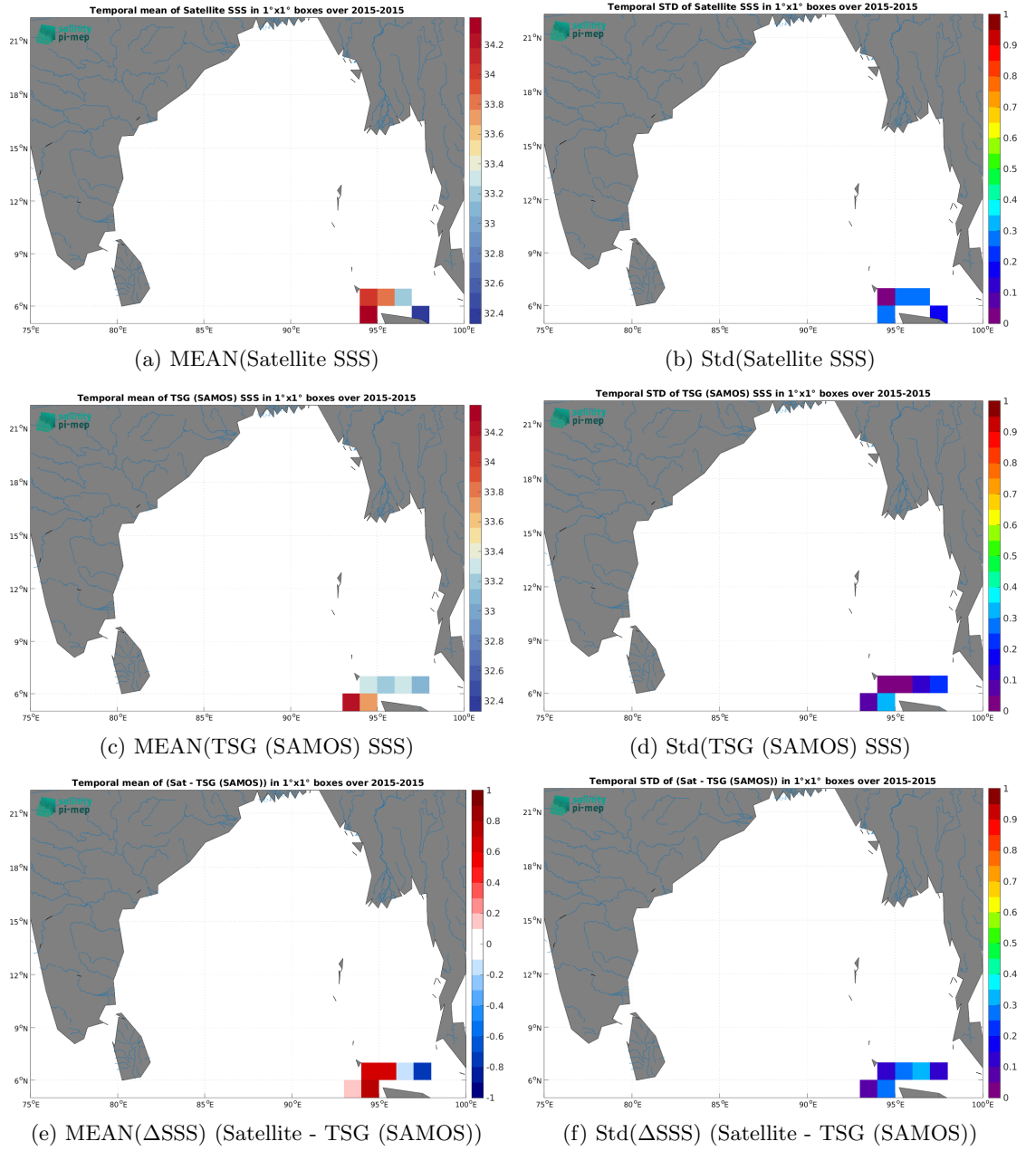
Figure 7: Temporal mean (left) and Std (right) of SSS from SMOS SSS L3 v335 - 10 Days - 25 km (CATDS-CPDC) (top), TSG (SAMOS) (middle), and of \Delta SSS (Satellite - TSG (SAMOS)). Only match-up pairs are used to generate these maps.
