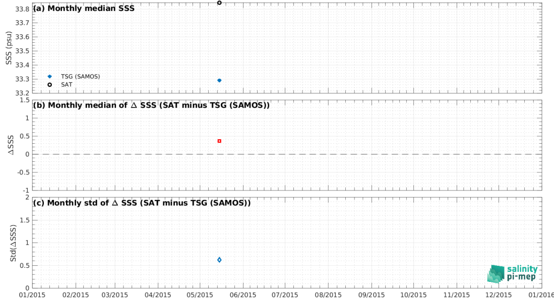
Figure 8: Time series of the monthly median SSS (top), median of \Delta SSS (Satellite - TSG (SAMOS)) and Std of \Delta SSS (Satellite - TSG (SAMOS)) over the Ganga and Brahmaputra river plumes Pi-MEP region considering all match-ups collected by the Pi-MEP.
