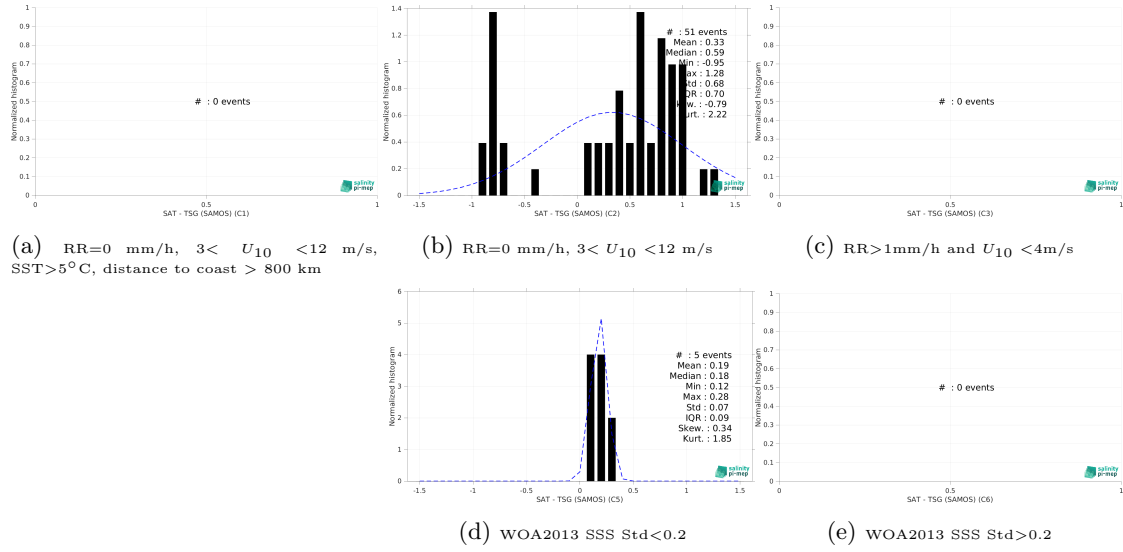
Figure 15: Normalized histogram of \Delta\text{SSS} (SMOS SSS L3 v335 - 10 Days - 25 km (CATDS-CPDC) - TSG (SAMOS)) for 5 different subdatasets corresponding to: RR=0 mm/h, 3 < U_{10} < 12 m/s, SST > 5^\circ\text{C} , distance to coast > 800 km (a), RR=0 mm/h, 3 < U_{10} < 12 m/s (b), RR > 1 mm/h and U_{10} < 4 m/s (c), WOA2013 SSS Std < 0.2 (d), WOA2013 SSS Std > 0.2 (e).
