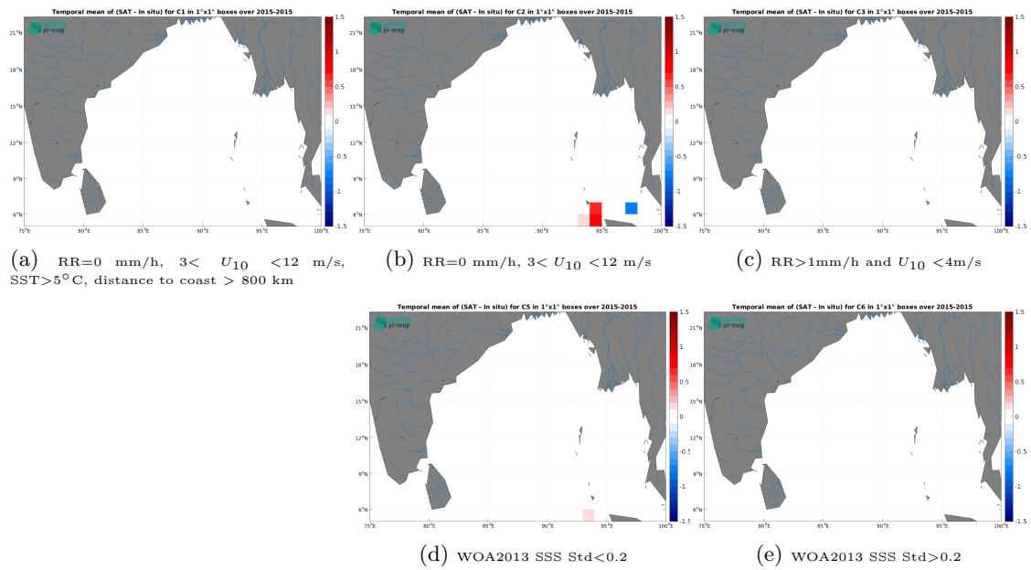
Figure 14: Temporal mean gridded over spatial boxes of size 1^\circ \times 1^\circ of \Delta SSS (SMOS SSS L3 v335 - 10 Days - 25 km (CATDS-CPDC) - TSG (SAMOS)) for 5 different subdatasets corresponding to: RR=0 mm/h, 3 < U_{10} < 12 m/s, SST > 5^\circ C , distance to coast > 800 km (a), RR=0 mm/h, 3 < U_{10} < 12 m/s (b), RR > 1 mm/h and U_{10} < 4 m/s (c), WOA2013 SSS Std < 0.2 (d), WOA2013 SSS Std > 0.2 (e).
