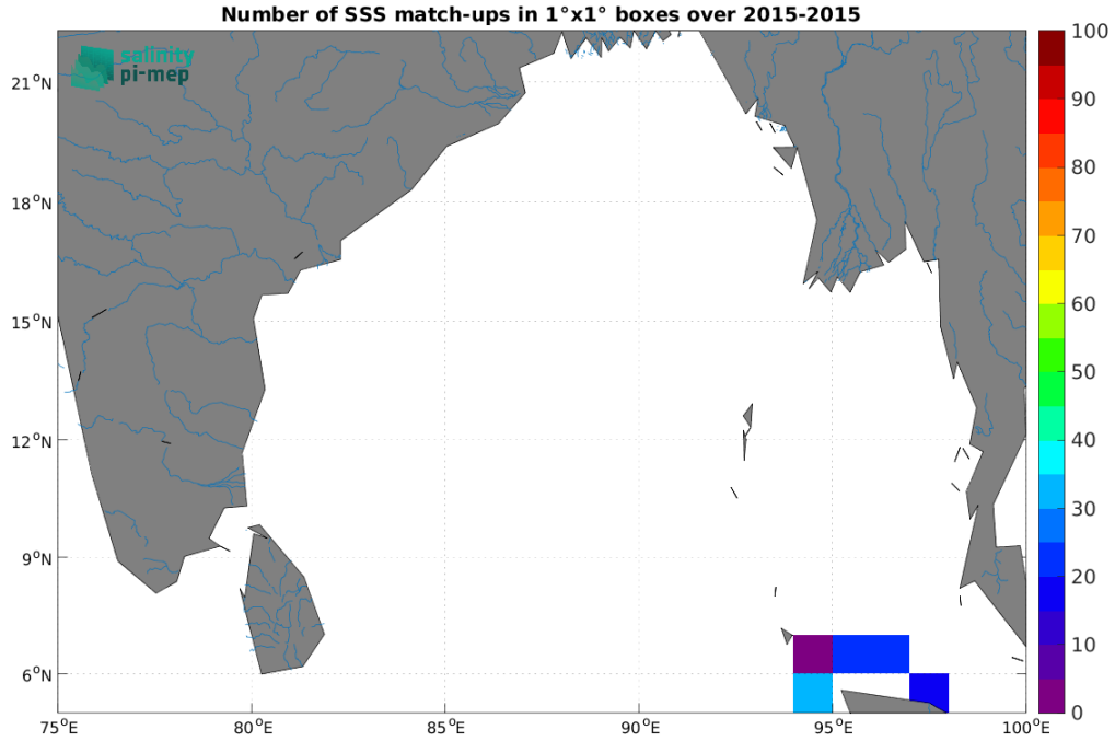
Figure 5: Number of SSS match-ups between TSG (SAMOS) SSS and the SMOS SSS L3 v335 - 10 Days - 25 km (CATDS-CPDC) SSS product for the Ganga and Brahmaputra river plumes Pi-MEP region over 1^\circ \times 1^\circ boxes and for the full satellite product period.
