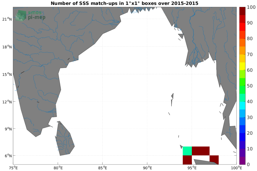
Figure 4: Number of SSS match-ups between TSG (SAMOS) SSS and the SMOS SSS L3 v335 - 10 Days - 25 km (CATDS-CPDC) SSS product for the Ganga and Brahmaputra river plumes Pi-MEP region over 1°x1° boxes and for the full satellite product period.
