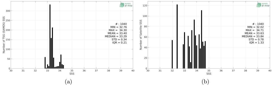
Figure 2: Histograms of SSS from TSG (SAMOS) (a) and SMOS SSS L3 v335 - 10 Days - 25 km (CATDS-CPDC) (b) considering all match-up pairs per bins of 0.1 over the Ganga and Brahmaputra river plumes Pi-MEP region and for the full satellite product period.
