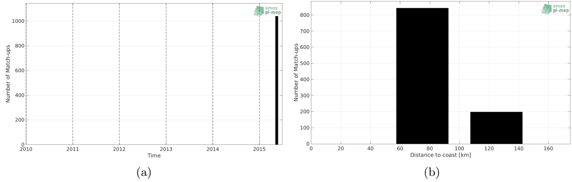
Figure 1: Number of match-ups between TSG (SAMOS) and SMOS SSS L3 v335 - 10 Days - 25 km (CATDS-CPDC) SSS as a function of time (a) and as function of the distance to coast (b) over the Ganga and Brahmaputra river plumes Pi-MEP region and for the full satellite product period.
