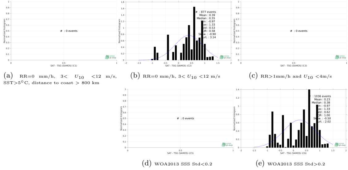
Figure 13: Normalized histogram of \Delta\text{SSS} (SMOS SSS L3 v335 - 10 Days - 25 km (CATDS-CPDC) - TSG (SAMOS)) for 5 different subdatasets corresponding to: RR=0 mm/h, 3 < U_{10} < 12 m/s, SST > 5^\circ\text{C} , distance to coast > 800 km (a), RR=0 mm/h, 3 < U_{10} < 12 m/s (b), RR > 1\text{mm/h} and U_{10} < 4\text{m/s} (c), WOA2013 SSS Std < 0.2 (d), WOA2013 SSS Std > 0.2 (e).
