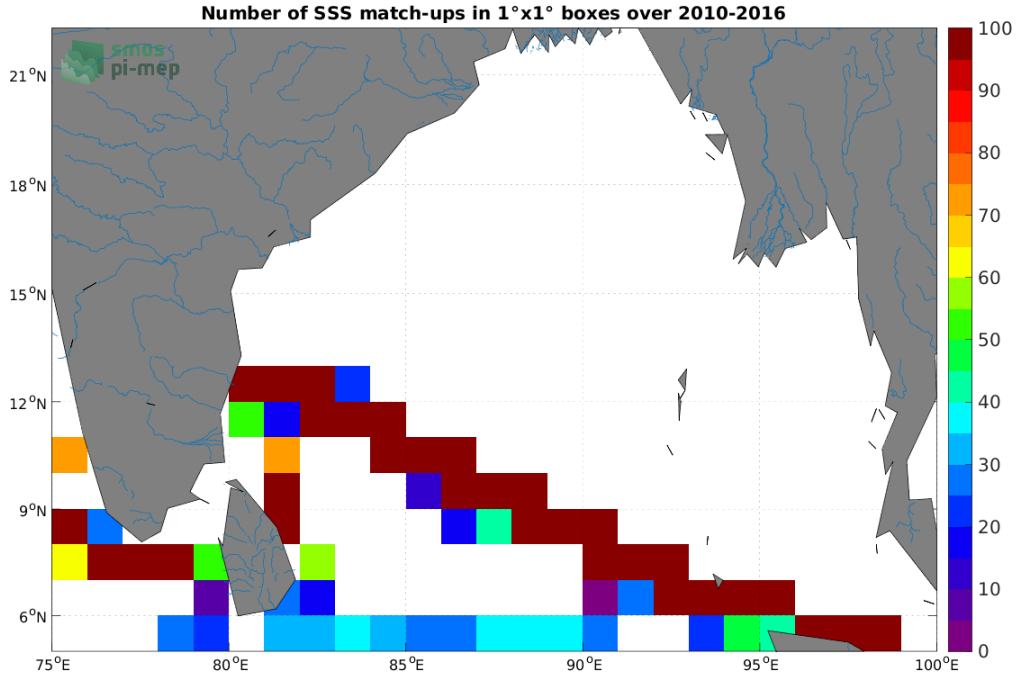
Figure 4: Number of SSS match-ups between TSG (LEGOS-DM) SSS and the SMOS SSS L3 v335 - 10 Days - 25 km (CATDS-CPDC) SSS product for the Ganga and Brahmaputra river plumes Pi-MEP region over 1°×1° boxes and for the full satellite product period.
