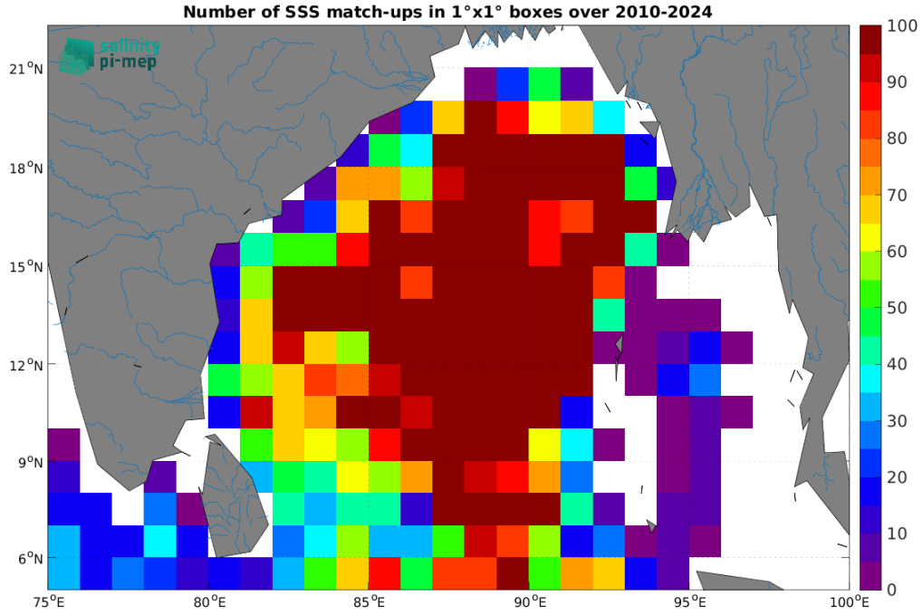
Figure 5: Number of SSS match-ups between Argo SSS and the SMOS SSS L3 v335 - 10 Days - 25 km (CATDS-CPDC) SSS product for the Ganga and Brahmaputra river plumes Pi-MEP region over 1^\circ \times 1^\circ boxes and for the full satellite product period.
