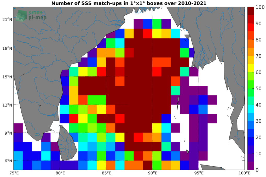
Figure 4: Number of SSS match-ups between Argo SSS and the SMOS SSS L3 v335 - 10 Days - 25 km (CATDS-CPDC) SSS product for the Ganga and Brahmaputra river plumes Pi-MEP region over 1^\circ \times 1^\circ boxes and for the full satellite product period.
