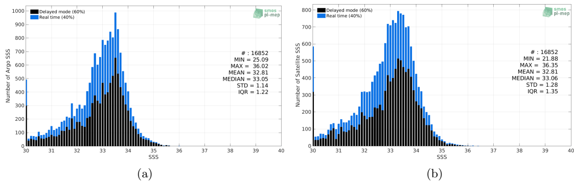
Figure 2: Histograms of SSS from Argo (a) and SMOS SSS L3 v335 - 10 Days - 25 km (CATDS-CPDC) (b) considering all match-up pairs per bins of 0.1 over the Ganga and Brahmaputra river plumes Pi-MEP region and for the full satellite product period.
