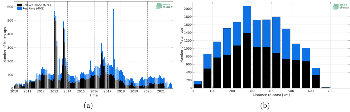
Figure 1: Number of match-ups between Argo and SMOS SSS L3 v335 - 10 Days - 25 km (CATDS-CPDC) SSS as a function of time (a) and as function of the distance to coast (b) over the Ganga and Brahmaputra river plumes Pi-MEP region and for the full satellite product period.
