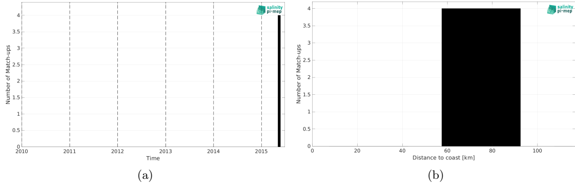
Figure 2: Number of match-ups between TSG (SAMOS) and SMOS SSS L2Q v333 - 0.25 Deg (CATDS-CPDC) SSS as a function of time (a) and as function of the distance to coast (b) over the Ganga and Brahmaputra river plumes Pi-MEP region and for the full satellite product period.
