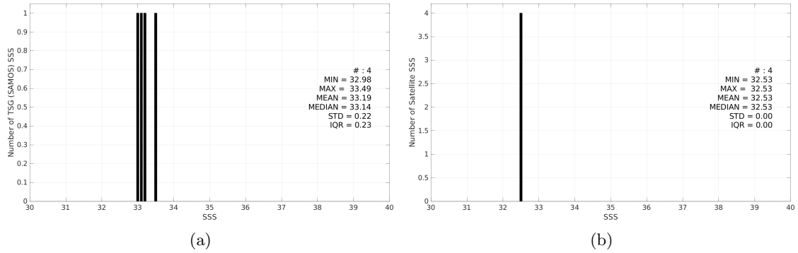
Figure 3: Histograms of SSS from TSG (SAMOS) (a) and SMOS SSS L2Q v333 - 0.25 Deg (CATDS-CPDC) (b) considering all match-up pairs per bins of 0.1 over the Ganga and Brahmaputra river plumes Pi-MEP region and for the full satellite product period.
