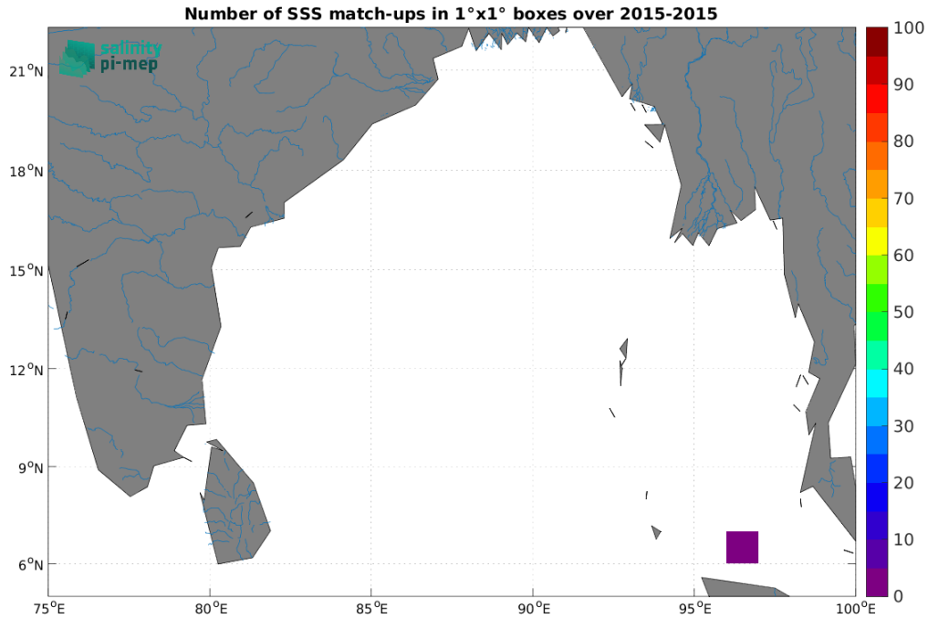
Figure 5: Number of SSS match-ups between TSG (SAMOS) SSS and the SMOS SSS L2Q v333 - 0.25 Deg (CATDS-CPDC) SSS product for the Ganga and Brahmaputra river plumes Pi-MEP region over 1^\circ \times 1^\circ boxes and for the full satellite product period.
