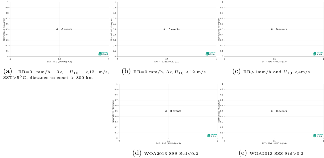
Figure 15: Normalized histogram of \Delta\text{SSS} (SMOS SSS L2Q v333 - 0.25 Deg (CATDS-CPDC) - TSG (SAMOS)) for 5 different subdatasets corresponding to: RR=0 mm/h, 3 < U_{10} < 12 m/s, SST > 5^\circ\text{C} , distance to coast > 800 km (a), RR=0 mm/h, 3 < U_{10} < 12 m/s (b), RR > 1 mm/h and U_{10} < 4 m/s (c), WOA2013 SSS Std < 0.2 (d), WOA2013 SSS Std > 0.2 (e).
