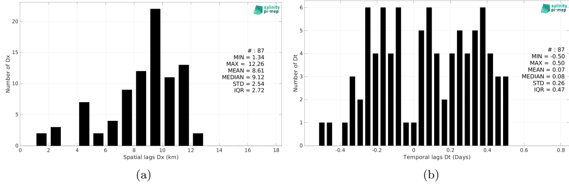
Figure 6: Histograms of the spatial (a) and temporal (b) lags between the location/time of the TSG (SAMOS) measurement and the date of the corresponding SMOS SSS L3 v332 - 9 Days (CATDS-CPDC) SSS pixel.
