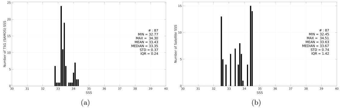
Figure 3: Histograms of SSS from TSG (SAMOS) (a) and SMOS SSS L3 v332 - 9 Days (CATDS-CPDC) (b) considering all match-up pairs per bins of 0.1 over the Ganga and Brahmaputra river plumes Pi-MEP region and for the full satellite product period.
