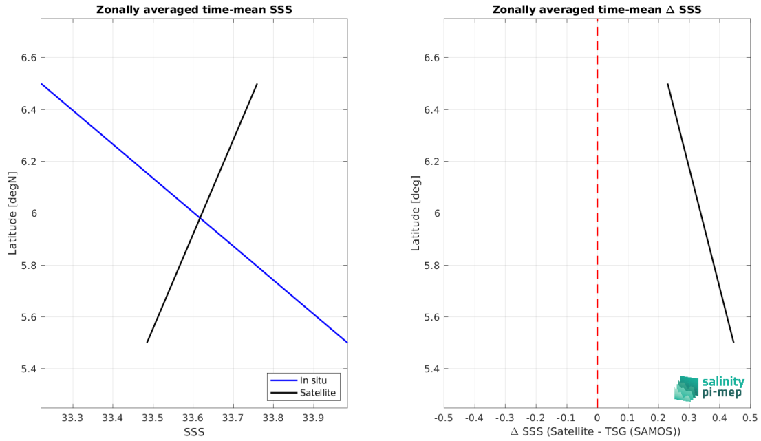
Figure 9: Left panel: Zonal mean SSS from SMOS SSS L3 v332 - 9 Days (CATDS-CPDC) satellite product (black) and from TSG (SAMOS) (blue). Right panel: Zonal mean of \Delta SSS (Satellite - TSG (SAMOS)) for all the collected Pi-MEP match-up pairs estimated over the full satellite product period.
