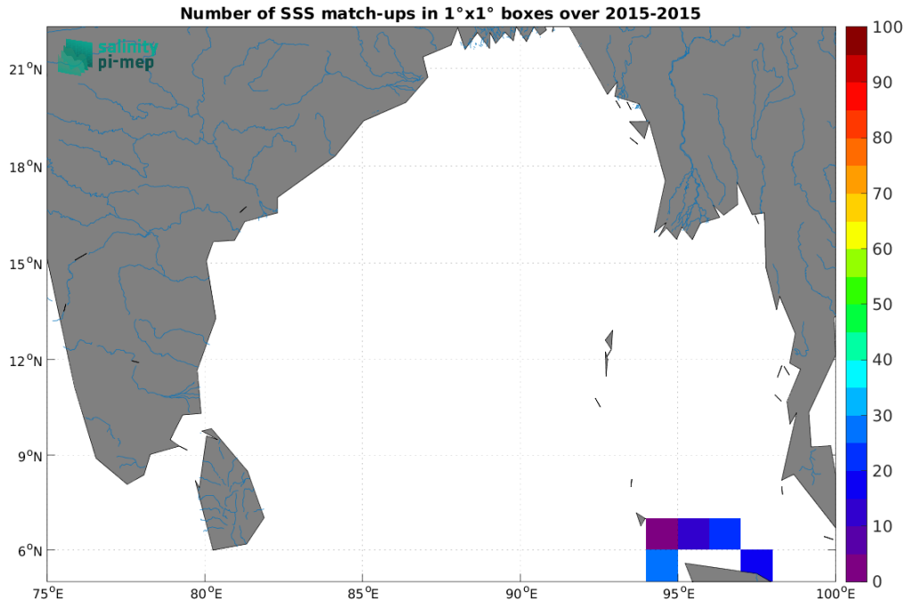
Figure 5: Number of SSS match-ups between TSG (SAMOS) SSS and the SMOS SSS L3 v332 - 9 Days (CATDS-CPDC) SSS product for the Ganga and Brahmaputra river plumes Pi-MEP region over 1^\circ \times 1^\circ boxes and for the full satellite product period.
