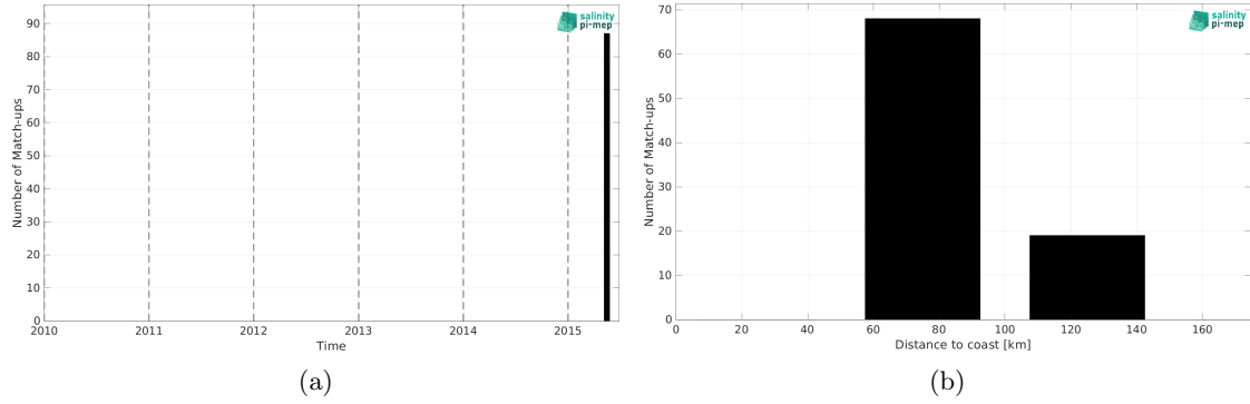
Figure 2: Number of match-ups between TSG (SAMOS) and SMOS SSS L3 v332 - 9 Days (CATDS-CPDC) SSS as a function of time (a) and as function of the distance to coast (b) over the Ganga and Brahmaputra river plumes Pi-MEP region and for the full satellite product period.
