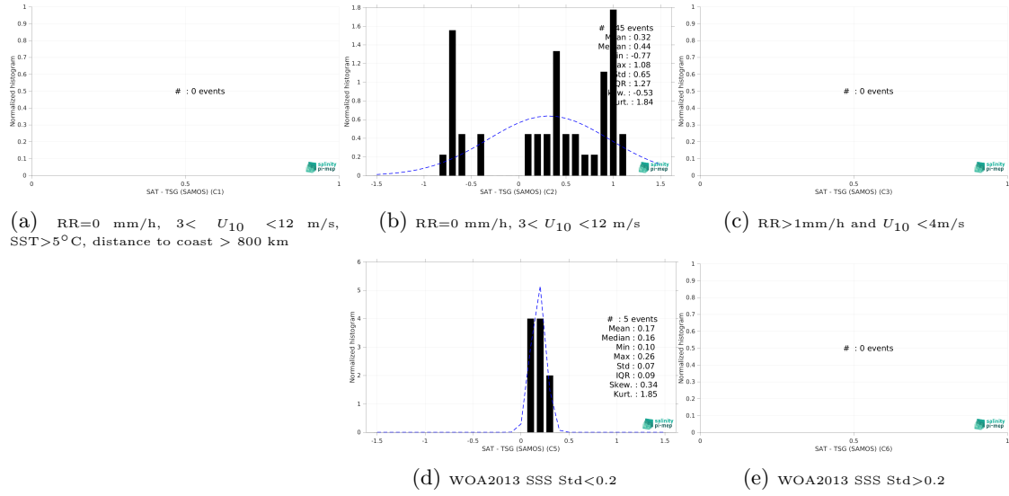
Figure 15: Normalized histogram of \Delta\text{SSS} (SMOS SSS L3 v332 - 9 Days (CATDS-CPDC) - TSG (SAMOS)) for 5 different subdatasets corresponding to: RR=0 mm/h, 3 < U_{10} < 12 m/s, SST > 5^\circ\text{C} , distance to coast > 800 km (a), RR=0 mm/h, 3 < U_{10} < 12 m/s, SST > 5^\circ\text{C} , distance to coast > 800 km (a), RR=0 mm/h, 3 < U_{10} < 12 m/s (b), RR > 1\text{mm/h} and U_{10} < 4\text{m/s} (c), WOA2013 SSS Std < 0.2 (d), WOA2013 SSS Std > 0.2 (e).
