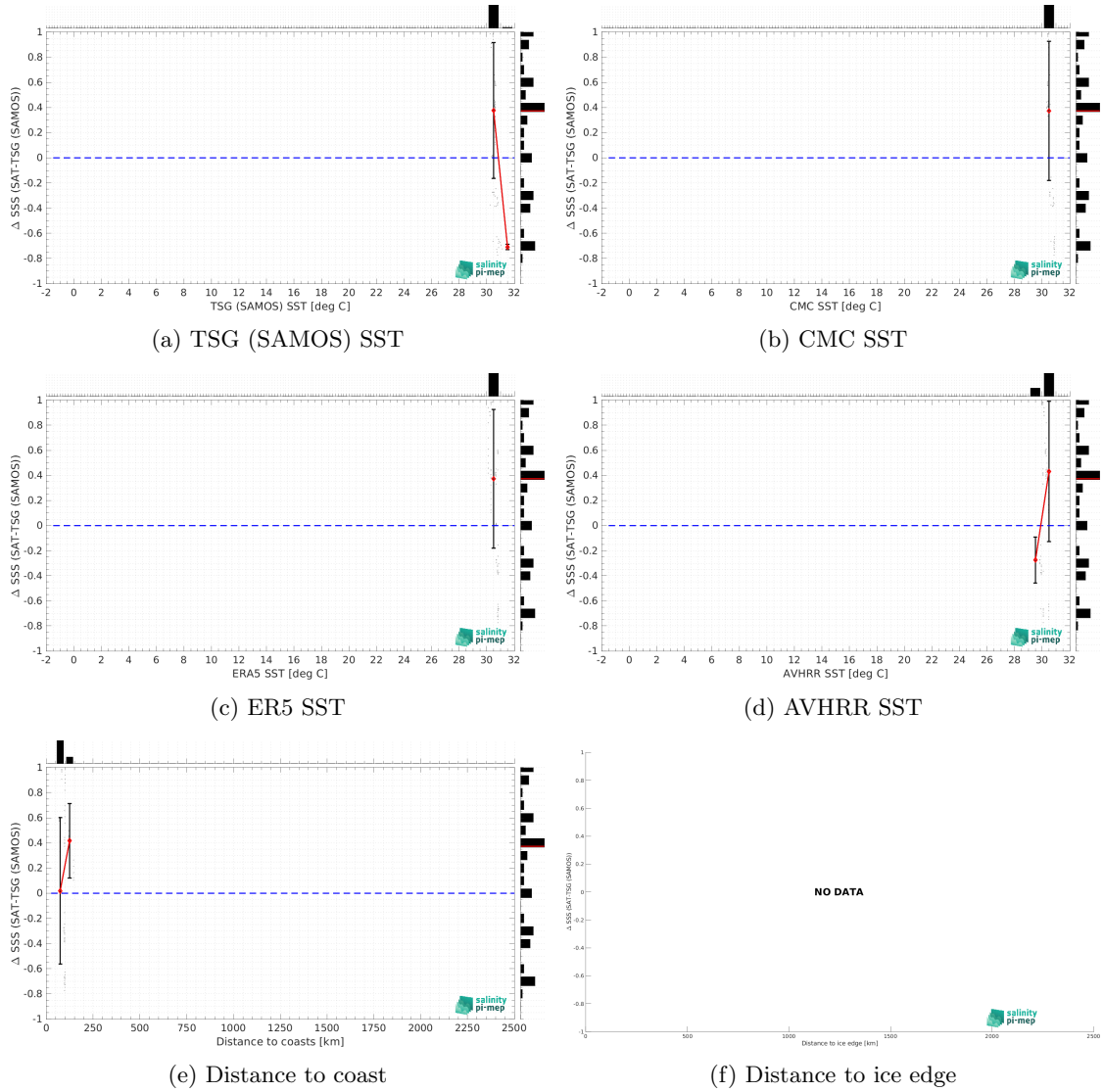
Figure 13: \Delta\text{SSS} (Satellite - TSG (SAMOS)) sorted as function of TSG (SAMOS) SST values (a), CMC SST (b), ERA5 SST (c), AVHRR SST (d), distance to coast (e) and distance to ice edge (f). In all plots the median and Std of \Delta\text{SSS} for each bin is indicated by the red curves and black vertical thick bars ( \pm 1 Std). Links to similar figures sorted as function of Sea ice fraction and in situ measurement depth .
