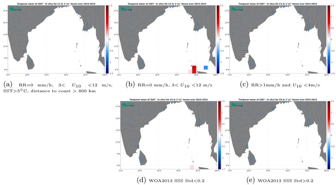
Figure 14: Temporal mean gridded over spatial boxes of size 1^\circ \times 1^\circ of \Delta SSS (SMOS SSS L3 v332 - 9 Days (CATDS-CPDC) - TSG (SAMOS)) for 5 different subdatasets corresponding to: RR=0 mm/h, 3 < U_{10} < 12 m/s, SST > 5^\circ C , distance to coast > 800 km (a), RR=0 mm/h, 3 < U_{10} < 12 m/s (b), RR > 1 mm/h and U_{10} < 4 m/s (c), WOA2013 SSS Std < 0.2 (d), WOA2013 SSS Std > 0.2 (e).
