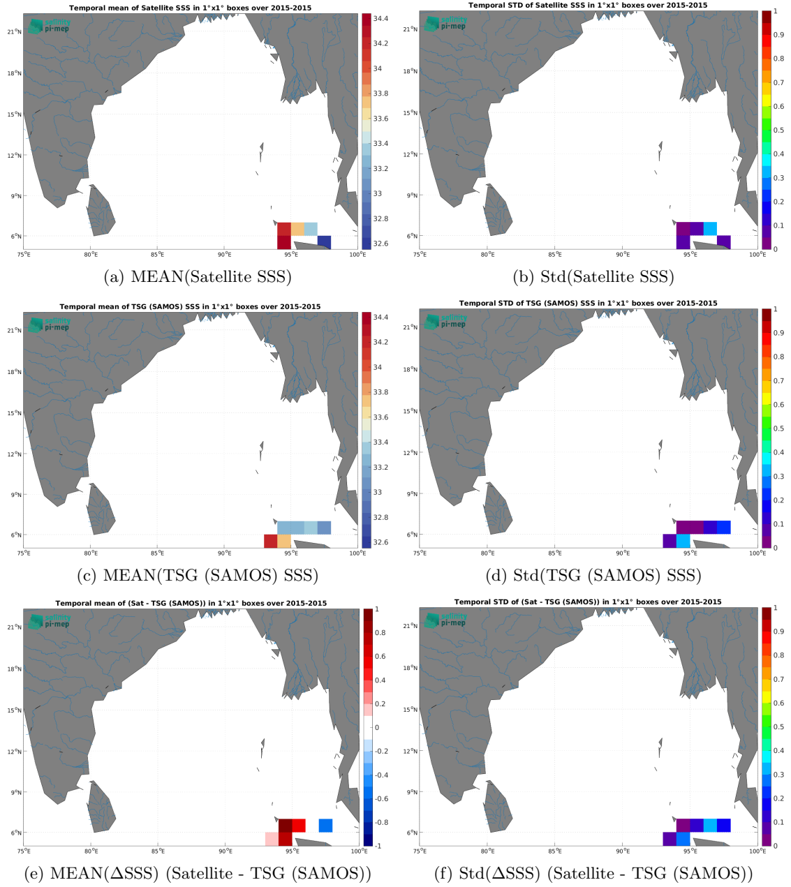
Figure 7: Temporal mean (left) and Std (right) of SSS from SMOS SSS L3 v332 - 9 Days (CATDS-CPDC) (top), TSG (SAMOS) (middle), and of \Delta SSS (Satellite - TSG (SAMOS)). Only match-up pairs are used to generate these maps.
