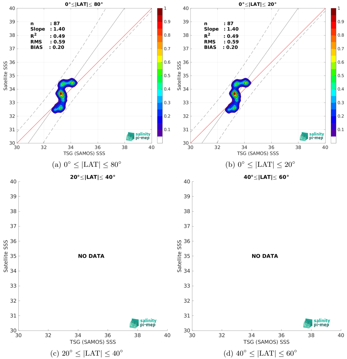
Figure 10: Contour maps of the concentration of SMOS SSS L3 v332 - 9 Days (CATDS-CPDC) SSS (y-axis) versus TSG (SAMOS) SSS (x-axis) at match-up pairs for different latitude bands. For each plot, the red line shows x=y . The black thin and dashed lines indicate a linear fit through the data cloud and the \pm 95\% confidence levels, respectively. The number match-up pairs n , the slope and R^2 coefficient of the linear fit, the root mean square (RMS) and the mean bias between satellite and in situ data are indicated for each latitude band in each plots.
