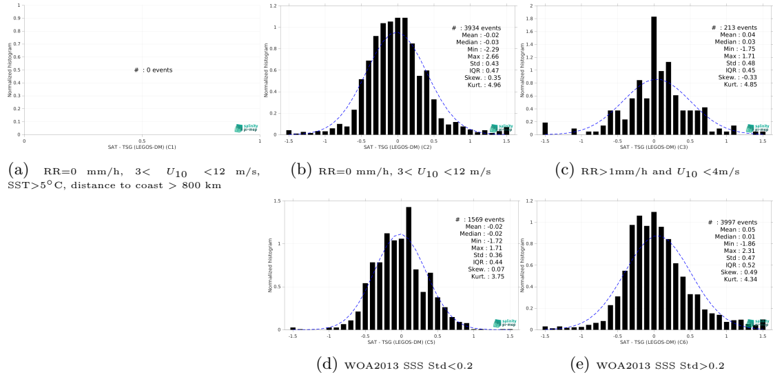
Figure 13: Normalized histogram of \Delta SSS (SMOS SSS L3 v332 - 9 Days (CATDS-CPDC) - TSG (LEGOS-DM)) for 5 different subdatasets corresponding to: RR=0 mm/h, 3 < U_{10} < 12 m/s, SST > 5^\circ C , distance to coast > 800 km (a), RR=0 mm/h, 3 < U_{10} < 12 m/s (b), RR > 1 mm/h and U_{10} < 4 m/s (c), WOA2013 SSS Std < 0.2 (d), WOA2013 SSS Std > 0.2 (e).
