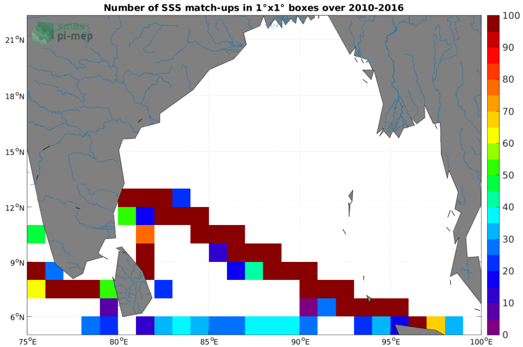
Figure 4: Number of SSS match-ups between TSG (LEGOS-DM) SSS and the SMOS SSS L3 v332 - 9 Days (CATDS-CPDC) SSS product for the Ganga and Brahmaputra river plumes Pi-MEP region over 1^\circ \times 1^\circ boxes and for the full satellite product period.
