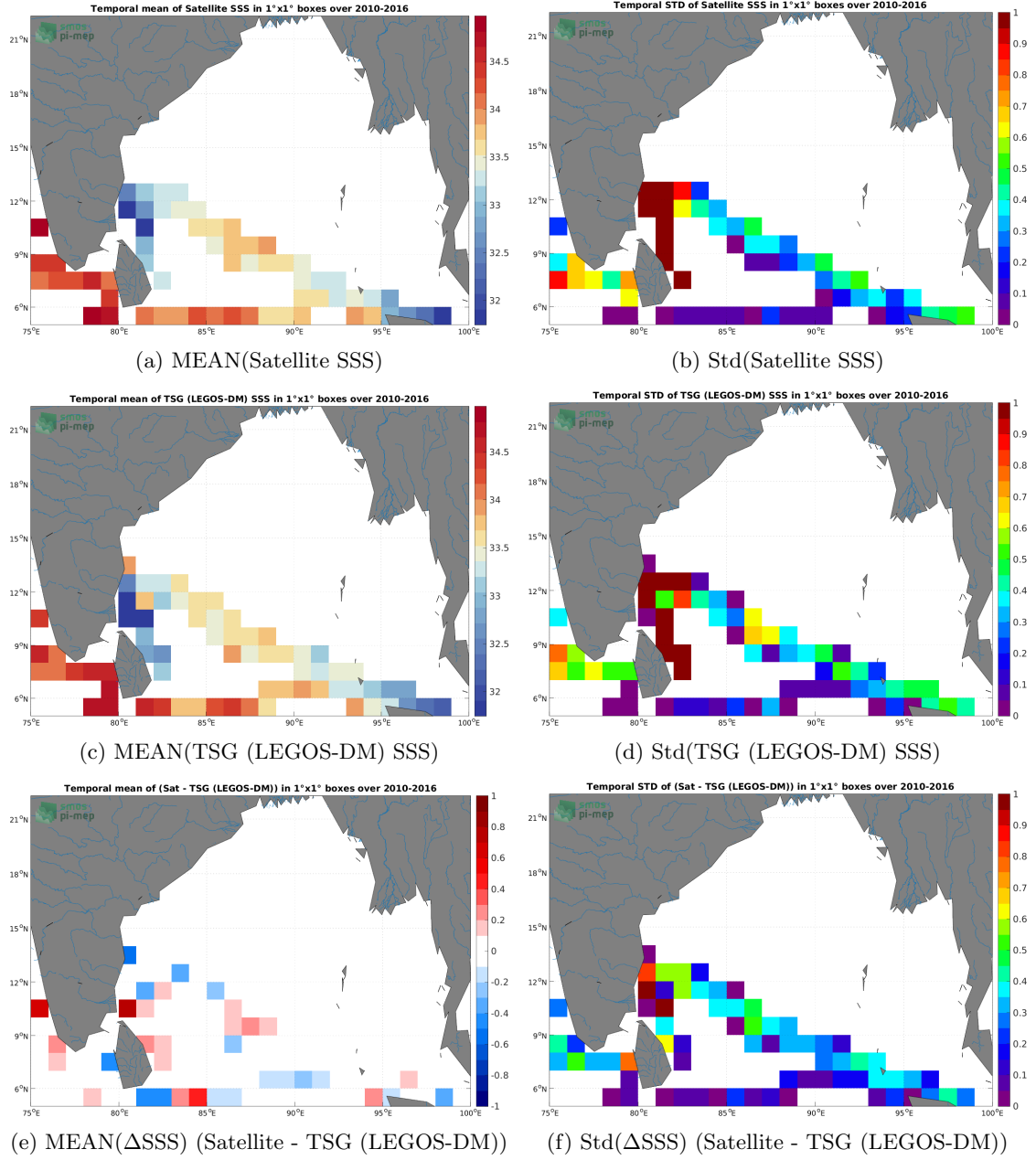
Figure 6: Temporal mean (left) and Std (right) of SSS from SMOS SSS L3 v332 - 9 Days (CATDS-CPDC) (top), TSG (LEGOS-DM) (middle), and of \Delta SSS (Satellite - TSG (LEGOS-DM)). Only match-up pairs are used to generate these maps.
