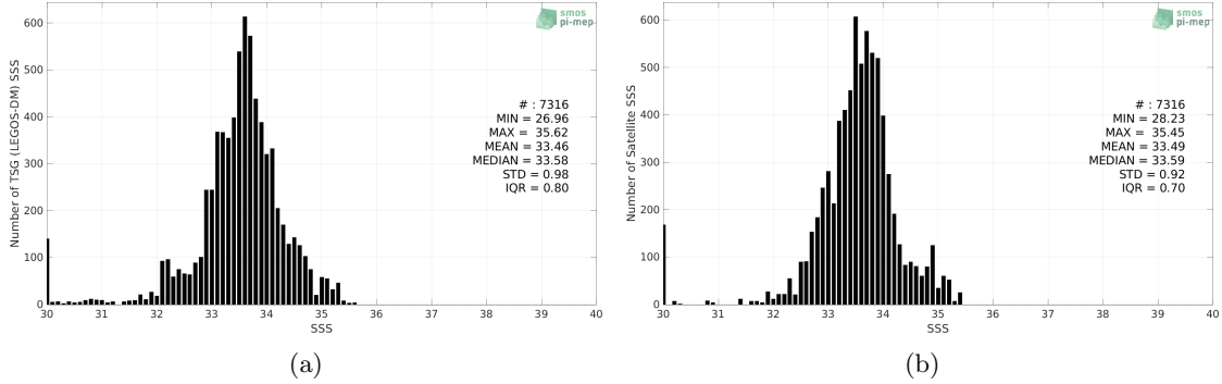
Figure 2: Histograms of SSS from TSG (LEGOS-DM) (a) and SMOS SSS L3 v332 - 9 Days (CATDS-CPDC) (b) considering all match-up pairs per bins of 0.1 over the Ganga and Brahmaputra river plumes Pi-MEP region and for the full satellite product period.
