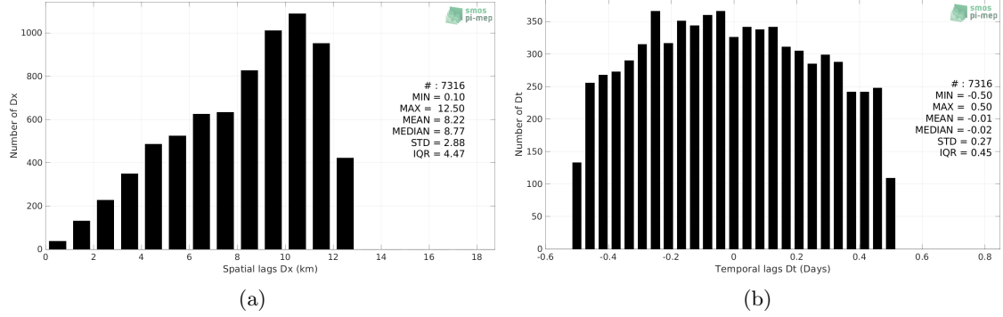
Figure 5: Histograms of the spatial (a) and temporal (b) lags between the location/time of the TSG (LEGOS-DM) measurement and the date of the corresponding SMOS SSS L3 v332 - 9 Days (CATDS-CPDC) SSS pixel.
