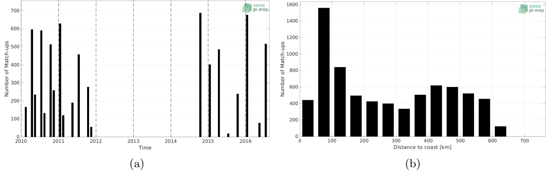
Figure 1: Number of match-ups between TSG (LEGOS-DM) and SMOS SSS L3 v332 - 9 Days (CATDS-CPDC) SSS as a function of time (a) and as function of the distance to coast (b) over the Ganga and Brahmaputra river plumes Pi-MEP region and for the full satellite product period.
