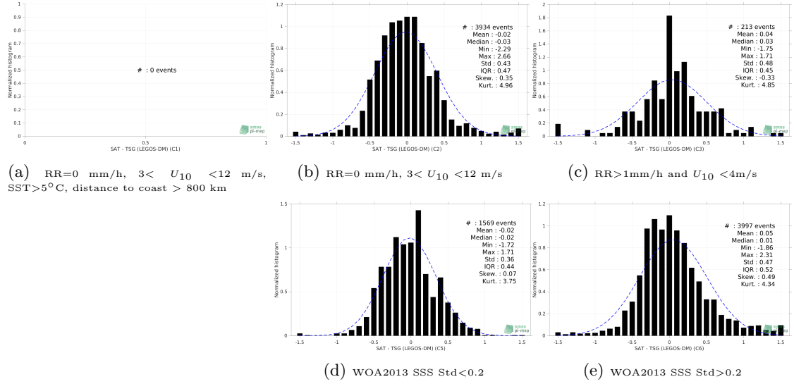
Figure 13: Normalized histogram of \Delta SSS (SMOS SSS L3 v332 - 9 Days (CATDS-CPDC) - TSG (LEGOS-DM)) for 5 different subdatasets corresponding to: RR=0 mm/h, 3 < U_{10} < 12 m/s, SST > 5^\circ C , distance to coast > 800 km (a), RR=0 mm/h, 3 < U_{10} < 12 m/s (b), RR > 1 mm/h and U_{10} < 4 m/s (c), WOA2013 SSS Std < 0.2 (d), WOA2013 SSS Std > 0.2 (e).
