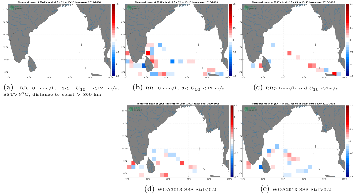
Figure 12: Temporal mean gridded over spatial boxes of size 1^\circ \times 1^\circ of \Delta SSS (SMOS SSS L3 v332 - 9 Days (CATDS-CPDC) - TSG (LEGOS-DM)) for 5 different subdatasets corresponding to: RR=0 mm/h, 3 < U_{10} < 12 m/s, SST > 5^\circ C , distance to coast > 800 km (a), RR=0 mm/h, 3 < U_{10} < 12 m/s (b), RR > 1 mm/h and U_{10} < 4 m/s (c), WOA2013 SSS Std < 0.2 (d), WOA2013 SSS Std > 0.2 (e).
