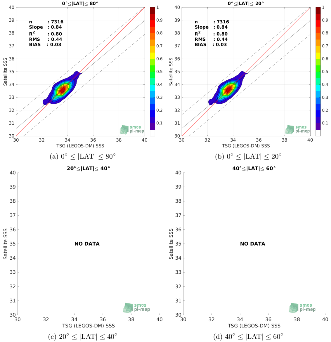
Figure 9: Contour maps of the concentration of SMOS SSS L3 v332 - 9 Days (CATDS-CPDC) SSS (y-axis) versus TSG (LEGOS-DM) SSS (x-axis) at match-up pairs for different latitude bands. For each plot, the red line shows x=y . The black thin and dashed lines indicate a linear fit through the data cloud and the \pm 95\% confidence levels, respectively. The number match-up pairs n , the slope and R^2 coefficient of the linear fit, the root mean square (RMS) and the mean bias between satellite and in situ data are indicated for each latitude band in each plots.
