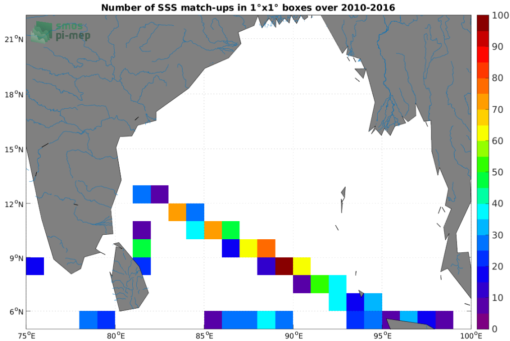
Figure 4: Number of SSS match-ups between TSG (LEGOS-DM) SSS and the SMOS SSS L2Q v331 - 0.25 Deg (CATDS-CPDC) SSS product for the Ganga and Brahmaputra river plumes Pi-MEP region over 1^\circ \times 1^\circ boxes and for the full satellite product period.
