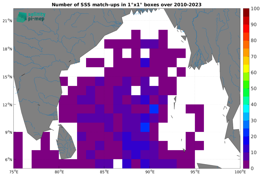
Figure 4: Number of SSS match-ups between Argo SSS and the SMOS SSS L2Q v331 - 0.25 Deg (CATDS-CPDC) SSS product for the Ganga and Brahmaputra river plumes Pi-MEP region over 1^\circ \times 1^\circ boxes and for the full satellite product period.
