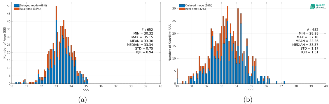
Figure 2: Histograms of SSS from Argo (a) and SMOS SSS L2Q v331 - 0.25 Deg (CATDS-CPDC) (b) considering all match-up pairs per bins of 0.1 over the Ganga and Brahmaputra river plumes Pi-MEP region and for the full satellite product period.
