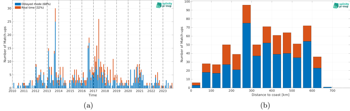
Figure 1: Number of match-ups between Argo and SMOS SSS L2Q v331 - 0.25 Deg (CATDS-CPDC) SSS as a function of time (a) and as function of the distance to coast (b) over the Ganga and Brahmaputra river plumes Pi-MEP region and for the full satellite product period.
