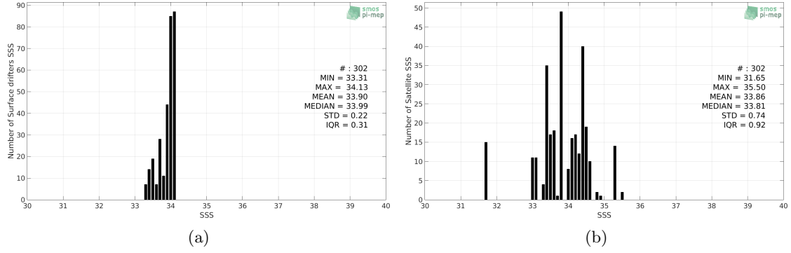
Figure 2: Histograms of SSS from Surface drifters (a) and SMOS SSS L2Q v321 - 0.25 Deg (CATDS-CPDC) (b) considering all match-up pairs per bins of 0.1 over the Ganga and Brahmaputra river plumes Pi-MEP region and for the full satellite product period.
