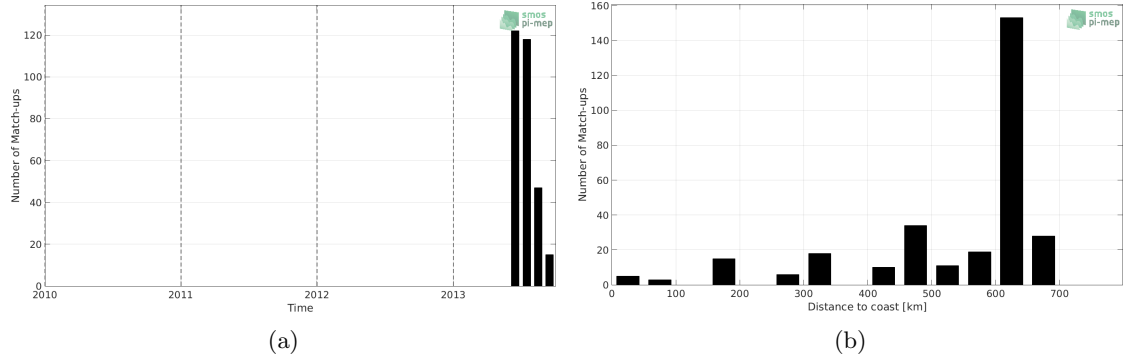
Figure 1: Number of match-ups between Surface drifters and SMOS SSS L2Q v321 - 0.25 Deg (CATDS-CPDC) SSS as a function of time (a) and as function of the distance to coast (b) over the Ganga and Brahmaputra river plumes Pi-MEP region and for the full satellite product period.
