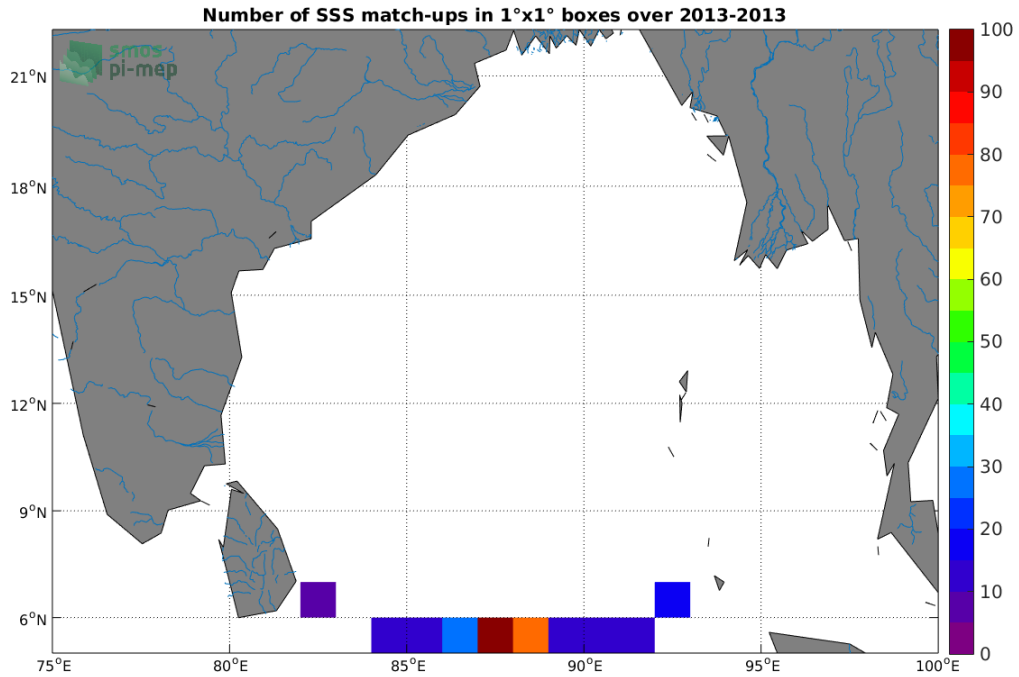
Figure 3: Number of SSS match-ups between Surface drifters SSS and the SMOS SSS L2Q v321 - 0.25 Deg (CATDS-CPDC) SSS product for the Ganga and Brahmaputra river plumes Pi-MEP region over 1^\circ \times 1^\circ boxes and for the full satellite product period.
