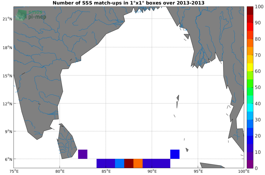
Figure 3: Number of SSS match-ups between Surface drifters SSS and the SMOS SSS L2Q v321 - 0.25 Deg (CATDS-CPDC) SSS product for the Ganga and Brahmaputra river plumes Pi-MEP region over 1°x1° boxes and for the full satellite product period.
