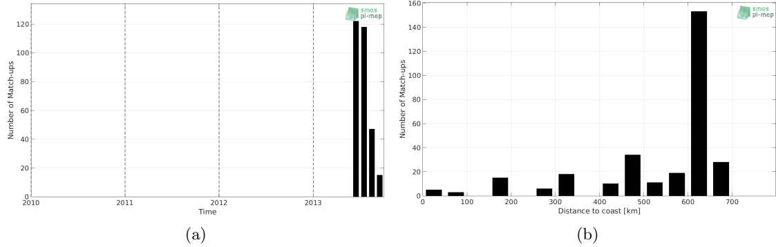
Figure 1: Number of match-ups between Surface drifters and SMOS L2Q v321 - 0.25 Deg (CATDS-CPDC) SSS as a function of time (a) and as function of the distance to coast (b) over the Ganga and Brahmaputra river plumes Pi-MEP region and for the full satellite product period.
