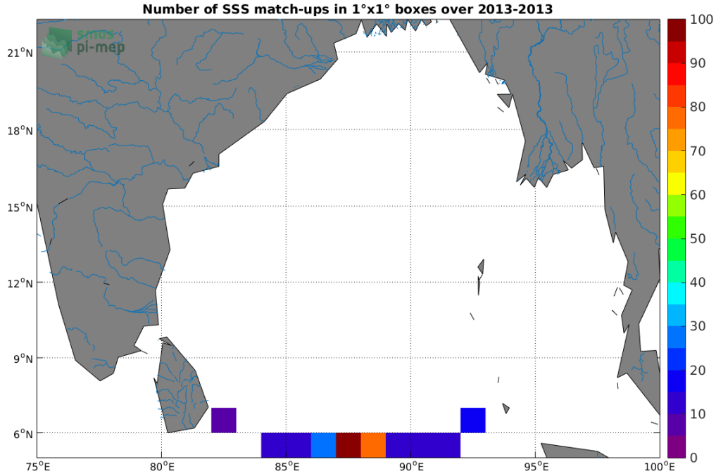
Figure 3: Number of SSS match-ups between Surface drifters SSS and the SMOS L2Q v321 - 0.25 Deg (CATDS-CPDC) SSS product for the Ganga and Brahmaputra river plumes Pi-MEP region over 1^\circ \times 1^\circ boxes and for the full satellite product period.
