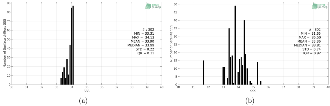
Figure 2: Histograms of SSS from Surface drifters (a) and SMOS L2Q v321 - 0.25 Deg (CATDS-CPDC) (b) considering all match-up pairs per bins of 0.1 over the Ganga and Brahmaputra river plumes Pi-MEP region and for the full satellite product period.
