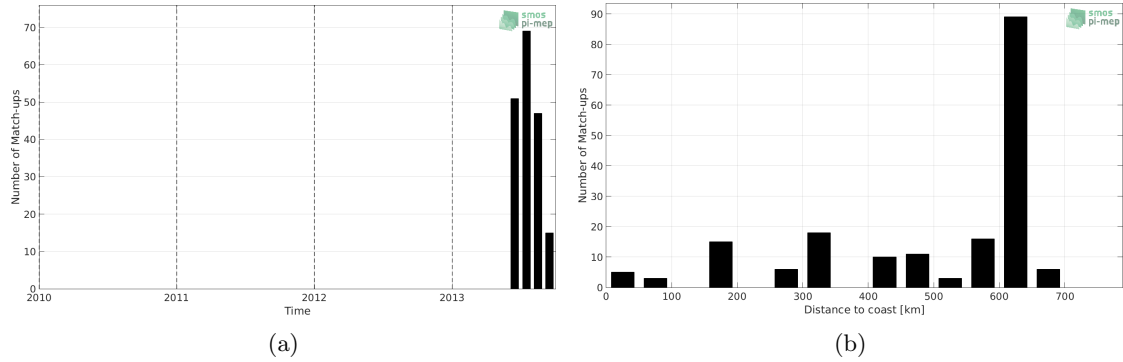
Figure 1: Number of match-ups between Surface drifters and SMOS-L3-CATDS-CPDC-V321-L2Q SSS as a function of time (a) and as function of the distance to coast (b) over the Ganga and Brahmaputra river plumes Pi-MEP region and for the full satellite product period.
