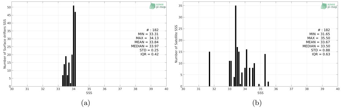
Figure 2: Histograms of SSS from Surface drifters (a) and SMOS-L3-CATDS-CPDC-V321-L2Q (b) considering all match-up pairs per bins of 0.1 over the Ganga and Brahmaputra river plumes Pi-MEP region and for the full satellite product period.
