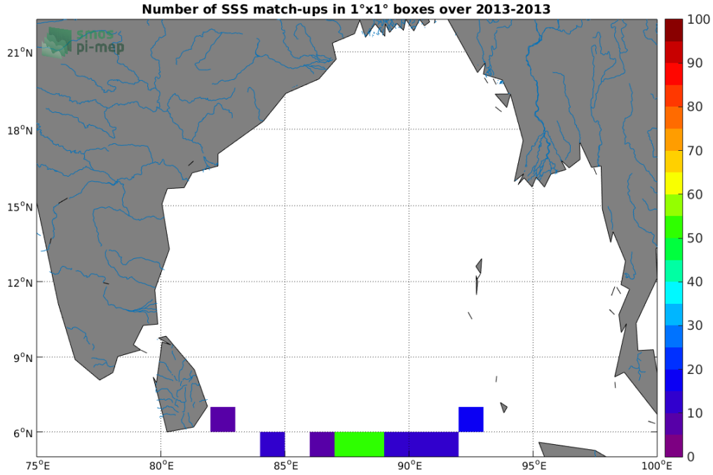
Figure 3: Number of SSS match-ups between Surface drifters SSS and the SMOS-L3-CATDS-CPDC-V321-L2Q SSS product for the Ganga and Brahmaputra river plumes Pi-MEP region over 1^\circ \times 1^\circ boxes and for the full satellite product period.
