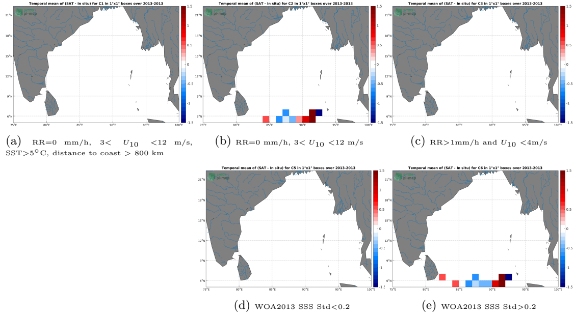
Figure 11: Temporal mean gridded over spatial boxes of size 1^\circ \times 1^\circ of \Delta SSS (SMOS-L3-CATDS-CPDC-V321-L2Q - Surface drifters) for 5 different subdatasets corresponding to: RR=0 mm/h, 3 < U_{10} < 12 m/s, SST > 5^\circ C , distance to coast > 800 km (a), RR=0 mm/h, 3 < U_{10} < 12 m/s (b), RR > 1 mm/h and U_{10} < 4 m/s (c), WOA2013 SSS Std < 0.2 (d), WOA2013 SSS Std > 0.2 (e).
