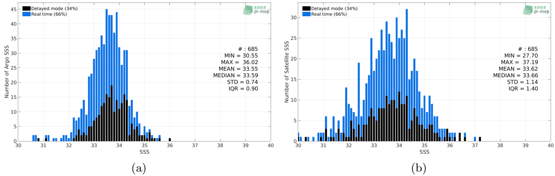
Figure 2: Histograms of SSS from Argo (a) and SMOS L2Q v321 - 0.25 Deg (CATDS-CPDC) (b) considering all match-up pairs per bins of 0.1 over the Ganga and Brahmaputra river plumes Pi-MEP region and for the full satellite product period.
