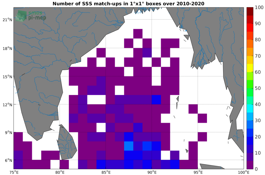
Figure 4: Number of SSS match-ups between Argo SSS and the SMOS L2Q v321 - 0.25 Deg (CATDS-CPDC) SSS product for the Ganga and Brahmaputra river plumes Pi-MEP region over 1°x1° boxes and for the full satellite product period.
