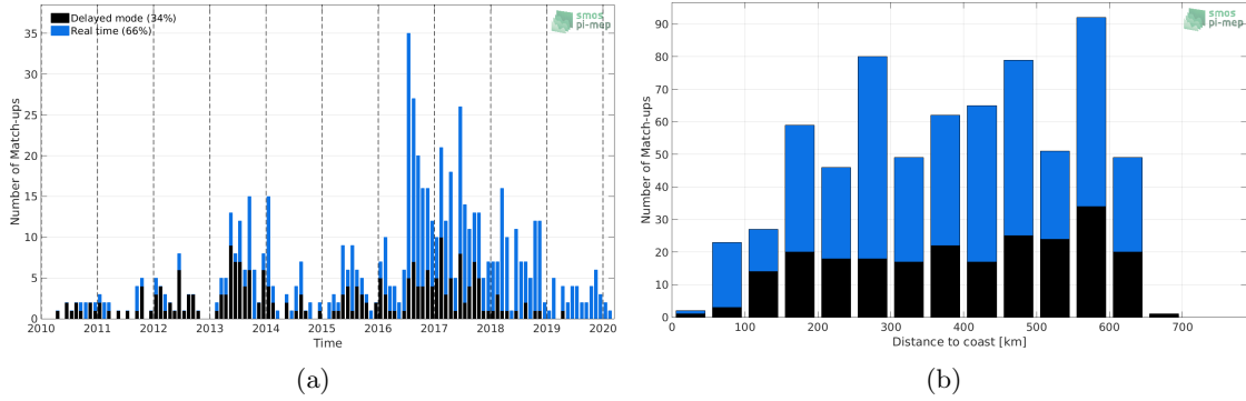
Figure 1: Number of match-ups between Argo and SMOS L2Q v321 - 0.25 Deg (CATDS-CPDC) SSS as a function of time (a) and as function of the distance to coast (b) over the Ganga and Brahmaputra river plumes Pi-MEP region and for the full satellite product period.
