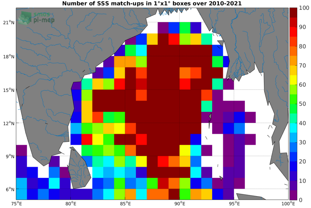
Figure 4: Number of SSS match-ups between Argo SSS and the SMOS SSS L3 v317 - Monthly - 25 km (CATDS-CPDC) SSS product for the Ganga and Brahmaputra river plumes Pi-MEP region over 1^\circ \times 1^\circ boxes and for the full satellite product period.
