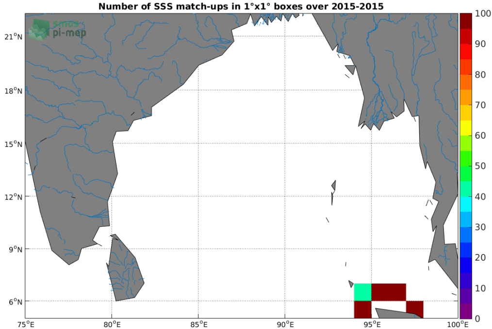
Figure 4: Number of SSS match-ups between TSG (SAMOS) SSS and the SMOS SSS L3 v317 - 10 Days - 25 km (CATDS-CPDC) SSS product for the Ganga and Brahmaputra river plumes Pi-MEP region over 1°×1° boxes and for the full satellite product period.
