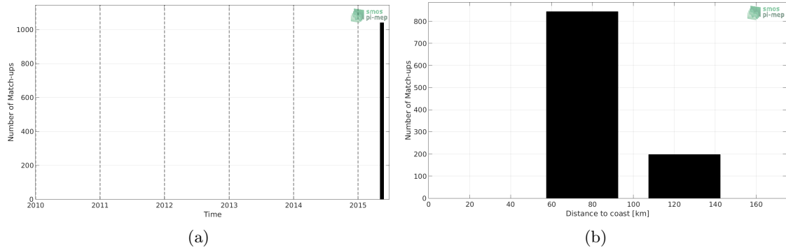
Figure 1: Number of match-ups between TSG-SAMOS and SMOS L3 v317 - 10 Days - 25 km (CATDS-CPDC) SSS as a function of time (a) and as function of the distance to coast (b) over the Ganga and Brahmaputra river plumes Pi-MEP region and for the full satellite product period.
