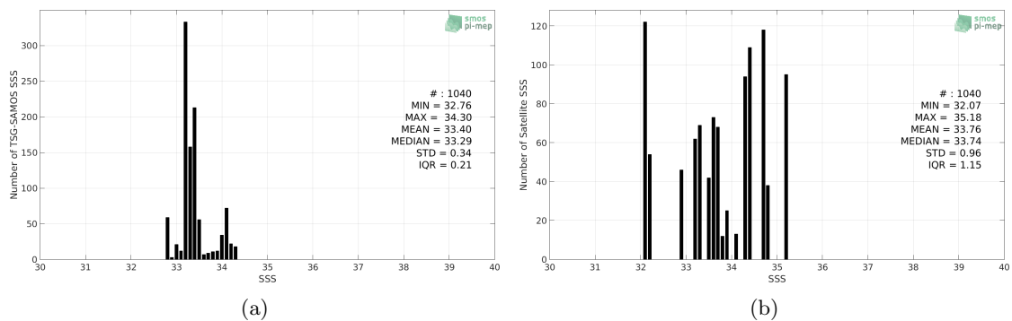
Figure 2: Histograms of SSS from TSG-SAMOS (a) and SMOS L3 v317 - 10 Days - 25 km (CATDS-CPDC) (b) considering all match-up pairs per bins of 0.1 over the Ganga and Brahmaputra river plumes Pi-MEP region and for the full satellite product period.
