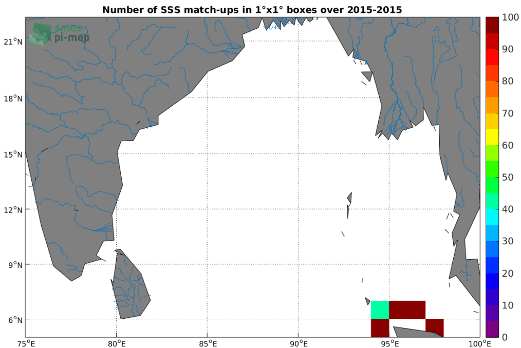
Figure 4: Number of SSS match-ups between TSG-SAMOS SSS and the SMOS-L3-CATDS-CPDC-V317-10DAYS-25KM SSS product for the Ganga and Brahmaputra river plumes Pi-MEP region over 1^{\circ} \times 1^{\circ} boxes and for the full satellite product period.
