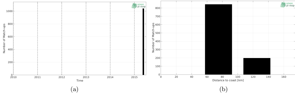
Figure 1: Number of match-ups between TSG-SAMOS and SMOS-L3-CATDS-CPDC-V317-10DAYS-25KM SSS as a function of time (a) and as function of the distance to coast (b) over the Ganga and Brahmaputra river plumes Pi-MEP region and for the full satellite product period.
