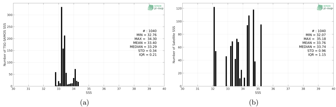
Figure 2: Histograms of SSS from TSG-SAMOS (a) and SMOS-L3-CATDS-CPDC-V317-10DAYS-25KM (b) considering all match-up pairs per bins of 0.1 over the Ganga and Brahmaputra river plumes Pi-MEP region and for the full satellite product period.
