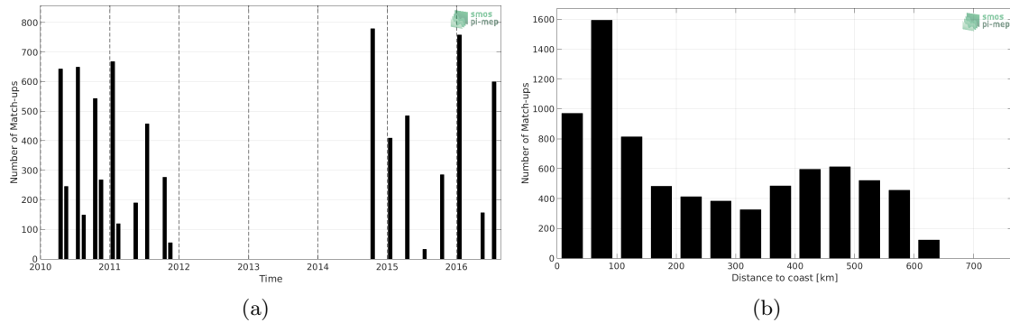
Figure 1: Number of match-ups between TSG (LEGOS-DM) and SMOS SSS L3 v317 - 10 Days - 25 km (CATDS-CPDC) SSS as a function of time (a) and as function of the distance to coast (b) over the Ganga and Brahmaputra river plumes Pi-MEP region and for the full satellite product period.
