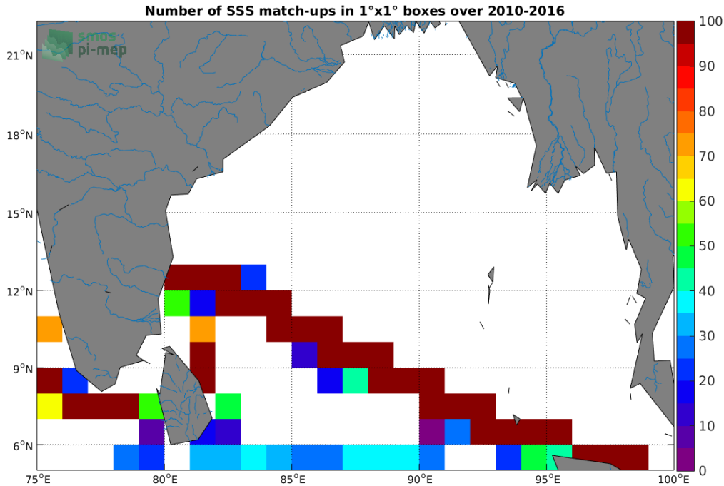
Figure 4: Number of SSS match-ups between TSG (LEGOS-DM) SSS and the SMOS SSS L3 v317 - 10 Days - 25 km (CATDS-CPDC) SSS product for the Ganga and Brahmaputra river plumes Pi-MEP region over 1^\circ \times 1^\circ boxes and for the full satellite product period.
