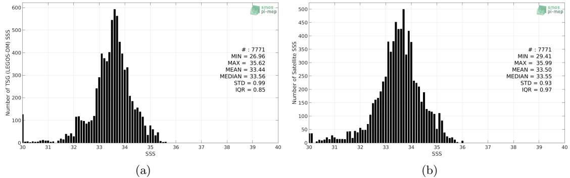
Figure 2: Histograms of SSS from TSG (LEGOS-DM) (a) and SMOS SSS L3 v317 - 10 Days - 25 km (CATDS-CPDC) (b) considering all match-up pairs per bins of 0.1 over the Ganga and Brahmaputra river plumes Pi-MEP region and for the full satellite product period.
