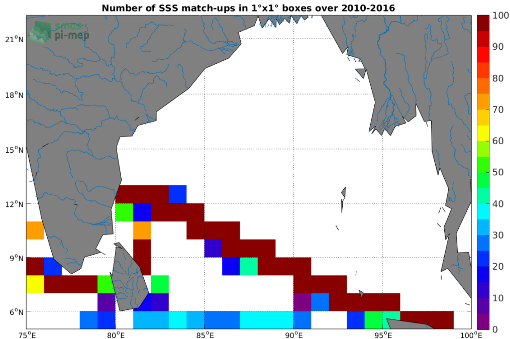
Figure 4: Number of SSS match-ups between TSG (LEGOS-DM) SSS and the SMOS SSS L3 v317 - 10 Days - 25 km (CATDS-CPDC) SSS product for the Ganga and Brahmaputra river plumes Pi-MEP region over 1°x1° boxes and for the full satellite product period.
