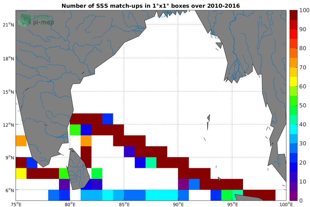
Figure 4: Number of SSS match-ups between TSG-LEGOS-DM SSS and the SMOS L3 v317 - 10 Days - 25 km (CATDS-CPDC) SSS product for the Ganga and Brahmaputra river plumes Pi-MEP region over 1^\circ \times 1^\circ boxes and for the full satellite product period.
