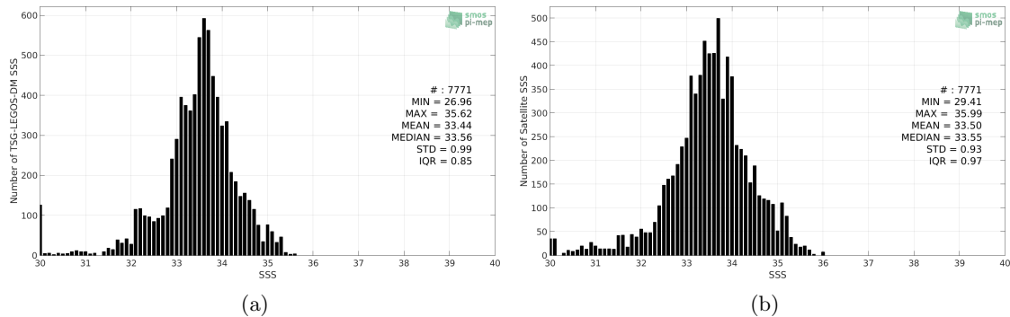
Figure 2: Histograms of SSS from TSG-LEGOS-DM (a) and SMOS L3 v317 - 10 Days - 25 km (CATDS-CPDC) (b) considering all match-up pairs per bins of 0.1 over the Ganga and Brahmaputra river plumes Pi-MEP region and for the full satellite product period.
