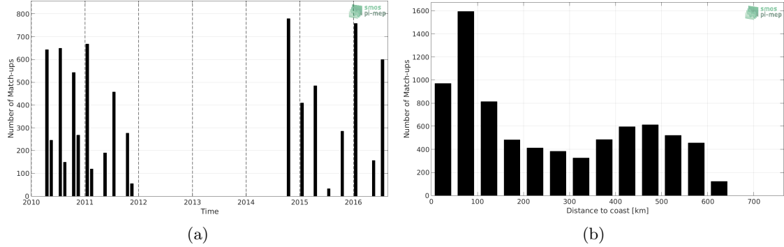
Figure 1: Number of match-ups between TSG-LEGOS-DM and SMOS L3 v317 - 10 Days - 25 km (CATDS-CPDC) SSS as a function of time (a) and as function of the distance to coast (b) over the Ganga and Brahmaputra river plumes Pi-MEP region and for the full satellite product period.
