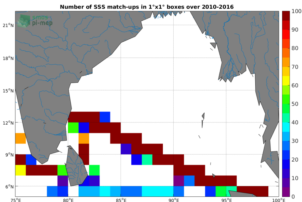
Figure 4: Number of SSS match-ups between TSG-LEGOS-DM SSS and the SMOS-L3-CATDS-CPDC-V317-10DAYS-25KM SSS product for the Ganga and Brahmaputra river plumes Pi-MEP region over 1°x1° boxes and for the full satellite product period.
