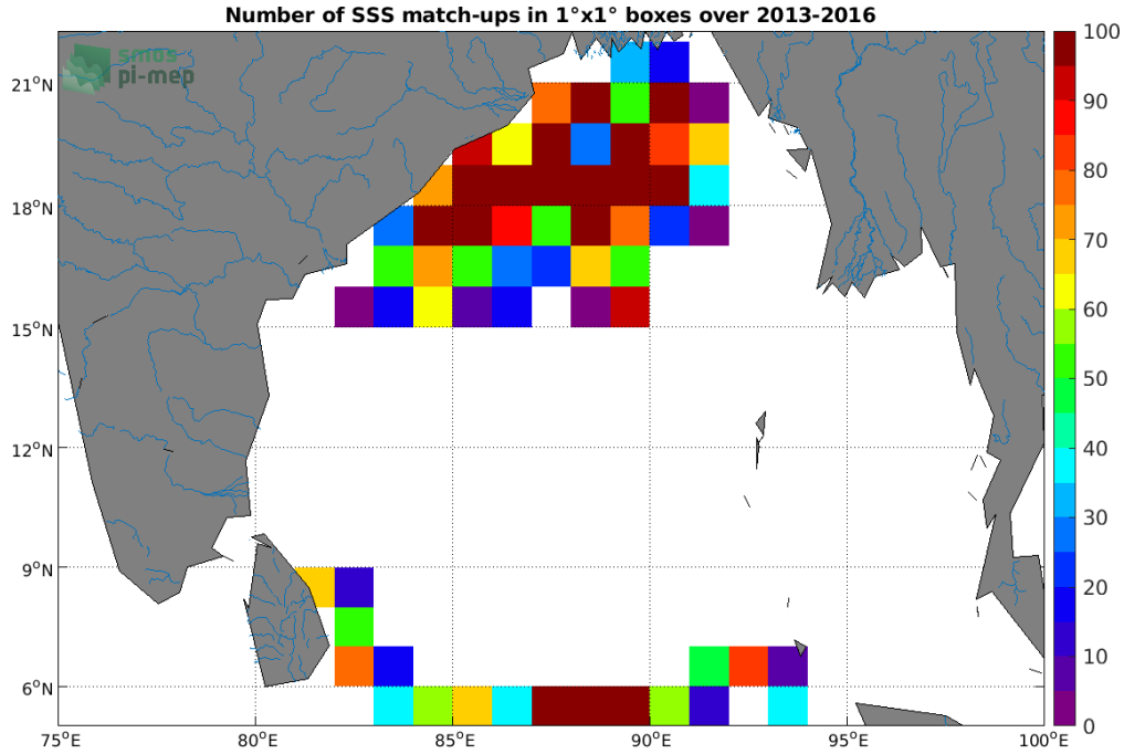
Figure 3: Number of SSS match-ups between Surface drifters SSS and the SMOS SSS L3 v317 - 10 Days - 25 km (CATDS-CPDC) SSS product for the Ganga and Brahmaputra river plumes Pi-MEP region over 1^\circ \times 1^\circ boxes and for the full satellite product period.
