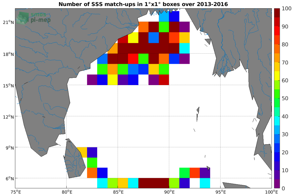
Figure 3: Number of SSS match-ups between Surface drifters SSS and the SMOS SSS L3 v317 - 10 Days - 25 km (CATDS-CPDC) SSS product for the Ganga and Brahmaputra river plumes Pi-MEP region over 1^{\circ} \times 1^{\circ} boxes and for the full satellite product period.
