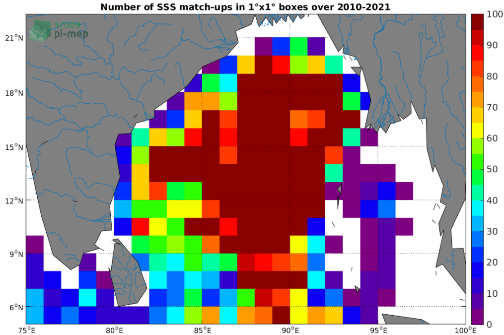
Figure 4: Number of SSS match-ups between Argo SSS and the SMOS SSS L3 v317 - 10 Days - 25 km (CATDS-CPDC) SSS product for the Ganga and Brahmaputra river plumes Pi-MEP region over 1°x1° boxes and for the full satellite product period.
