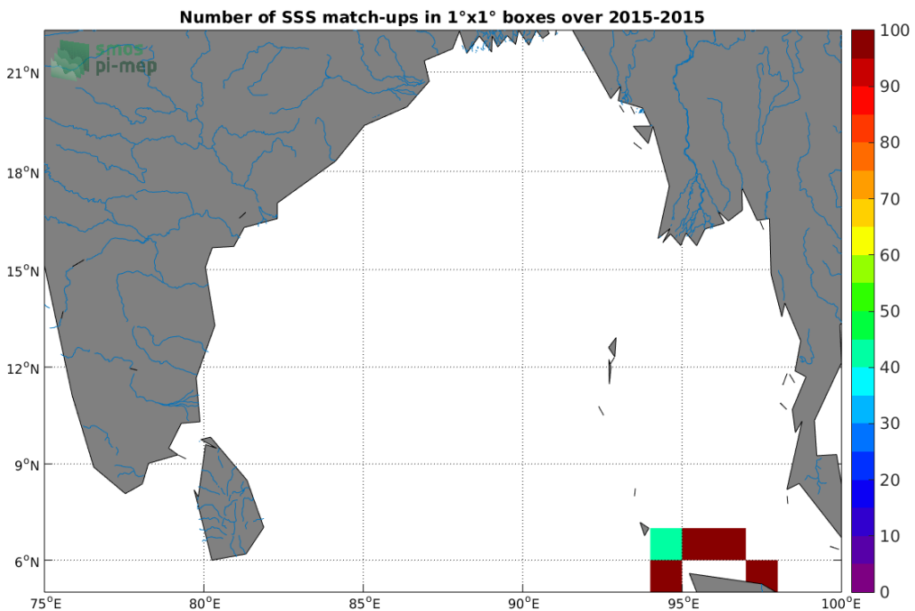
Figure 4: Number of SSS match-ups between TSG-SAMOS SSS and the SMOS-L3-CATDS-CPDC-V3-MONTHLY-25KM SSS product for the Ganga and Brahmaputra river plumes Pi-MEP region over 1°x1° boxes and for the full satellite product period.
