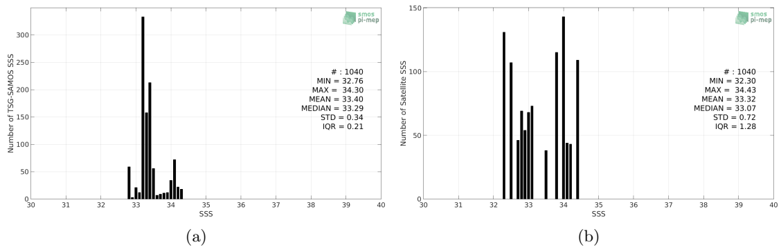
Figure 2: Histograms of SSS from TSG-SAMOS (a) and SMOS-L3-CATDS-CPDC-V3-MONTHLY-25KM (b) considering all match-up pairs per bins of 0.1 over the Ganga and Brahmaputra river plumes Pi-MEP region and for the full satellite product period.
