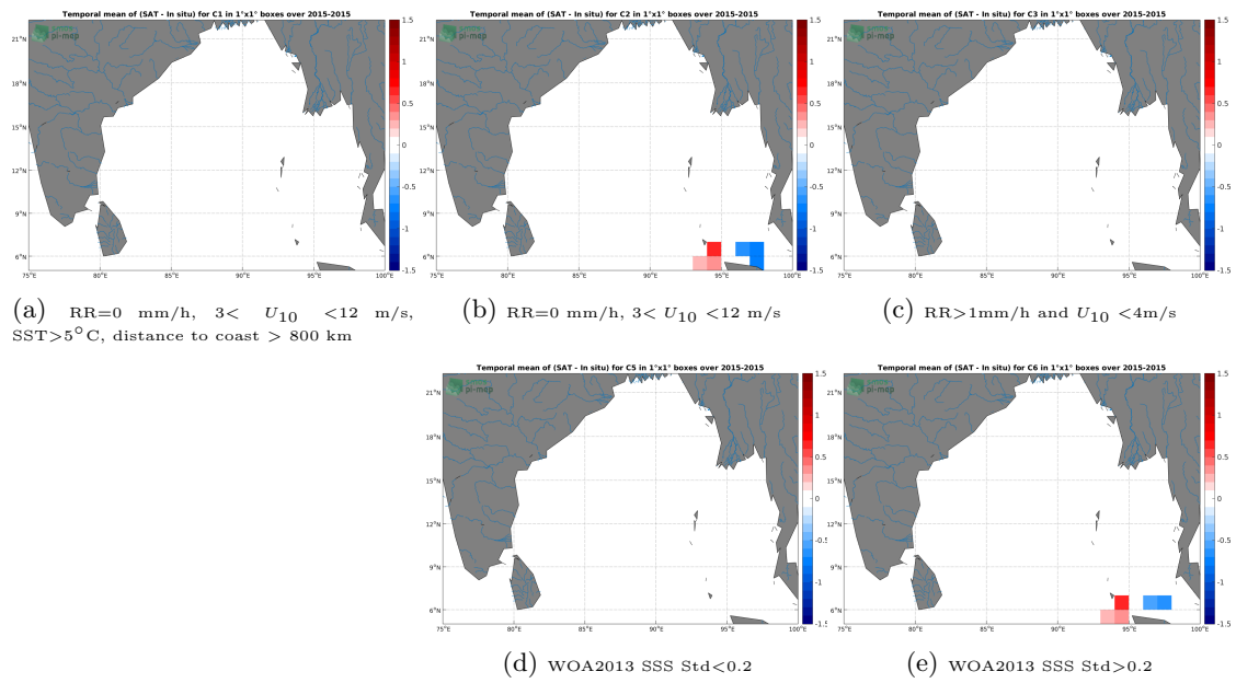
Figure 12: Temporal mean gridded over spatial boxes of size 1^\circ \times 1^\circ of \Delta SSS (SMOS-L3-CATDS-CPDC-V3-MONTHLY-25KM - TSG-SAMOS) for 5 different subdatasets corresponding to:RR=0 mm/h, 3 < U_{10} < 12 m/s, SST >5^\circ C, distance to coast > 800 km (a), RR=0 mm/h, 3 < U_{10} < 12 m/s (b), RR >1 mm/h and U_{10} < 4 m/s (c), WOA2013 SSS Std <0.2 (d), WOA2013 SSS Std >0.2 (e).
