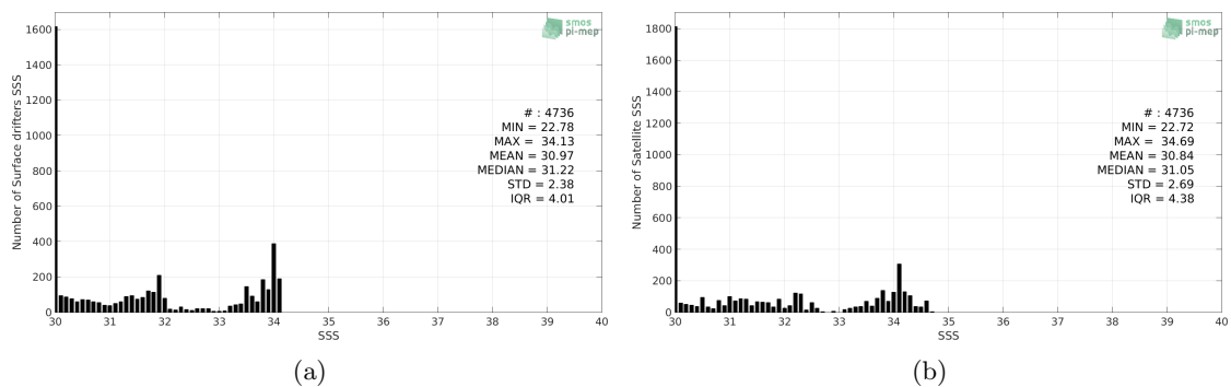
Figure 2: Histograms of SSS from Surface drifters (a) and SMOS-L3-CATDS-CPDC-V3-MONTHLY-25KM (b) considering all match-up pairs per bins of 0.1 over the Ganga and Brahmaputra river plumes Pi-MEP region and for the full satellite product period.
