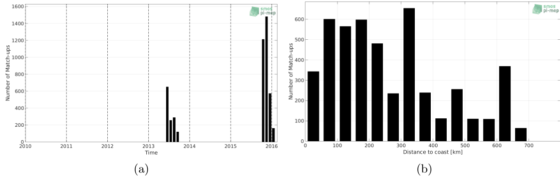
Figure 1: Number of match-ups between Surface drifters and SMOS-L3-CATDS-CPDC-V3-MONTHLY-25KM SSS as a function of time (a) and as function of the distance to coast (b) over the Ganga and Brahmaputra river plumes Pi-MEP region and for the full satellite product period.
