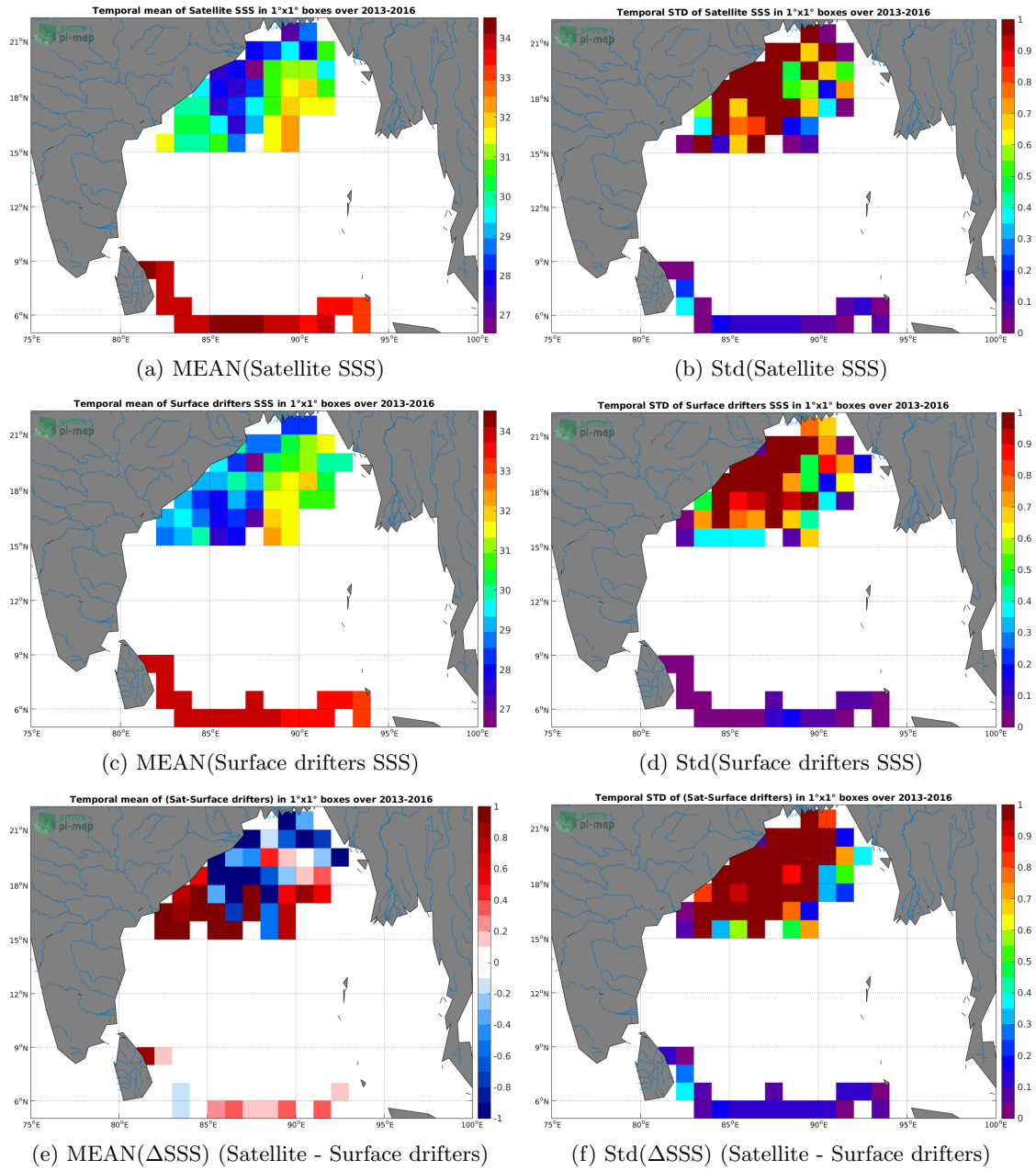
Figure 5: Temporal mean (left) and Std (right) of SSS from SMOS-L3-CATDS-CPDC-V3-MONTHLY-25KM (top), Surface drifters (middle), and of \Delta SSS (Satellite - Surface drifters). Only match-up pairs are used to generate these maps.
