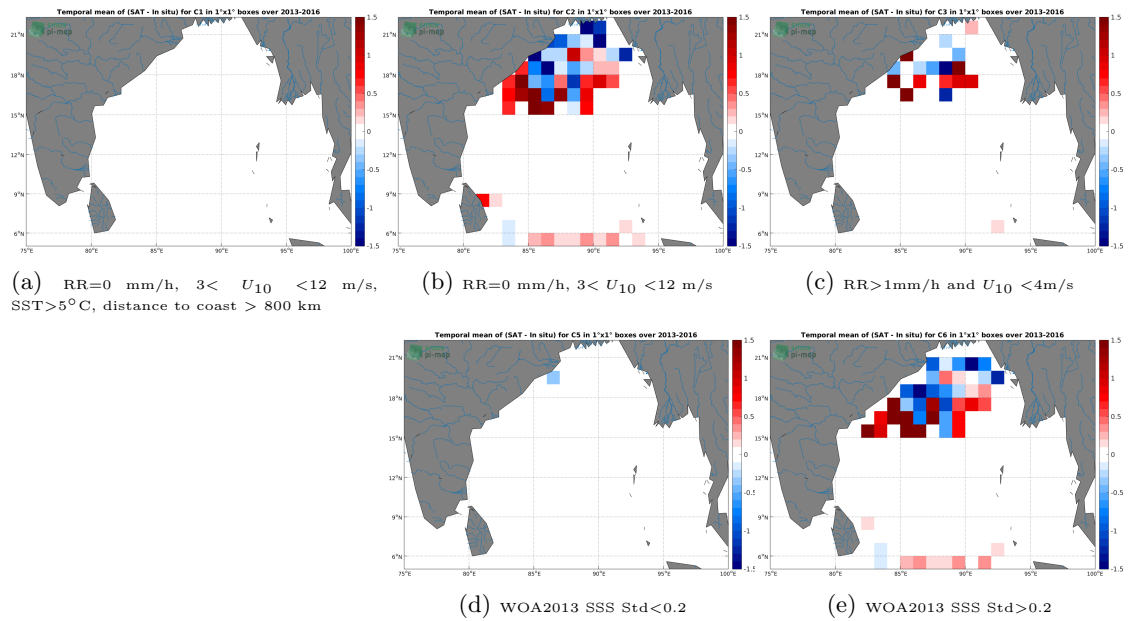
Figure 11: Temporal mean gridded over spatial boxes of size 1^\circ \times 1^\circ of \Delta SSS (SMOS-L3-CATDS-CPDC-V3-MONTHLY-25KM - Surface drifters) for 5 different subdatasets corresponding to:RR=0 mm/h, 3 < U_{10} < 12 m/s, SST >5^\circ C, distance to coast > 800 km (a), RR=0 mm/h, 3 < U_{10} < 12 m/s (b), RR >1 mm/h and U_{10} < 4 m/s (c), WOA2013 SSS Std <0.2 (d), WOA2013 SSS Std >0.2 (e).
