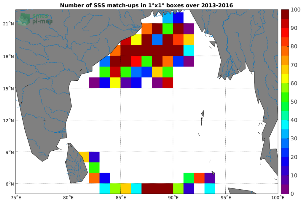
Figure 3: Number of SSS match-ups between Surface drifters SSS and the SMOS-L3-CATDS-CPDC-V3-MONTHLY-25KM SSS product for the Ganga and Brahmaputra river plumes Pi-MEP region over 1°x1° boxes and for the full satellite product period.
