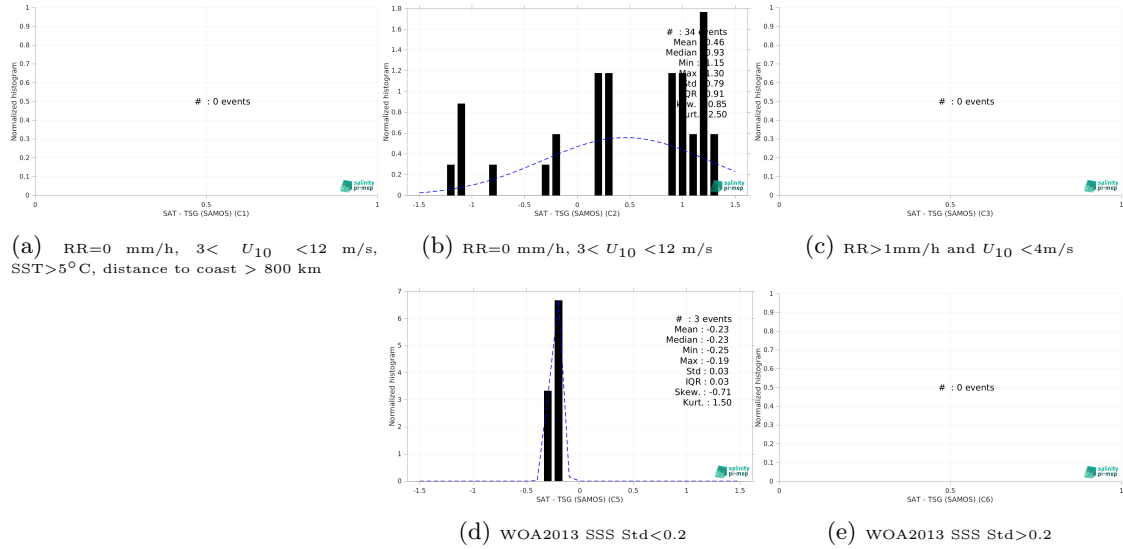
Figure 15: Normalized histogram of \Delta\text{SSS} (SMOS SSS L3 v2 - 9-Days (BEC) - TSG (SAMOS)) for 5 different subdatasets corresponding to: RR=0 mm/h, 3 < U_{10} < 12 m/s, SST > 5°C, distance to coast > 800 km (a), RR=0 mm/h, 3 < U_{10} < 12 m/s (b), RR > 1mm/h and U_{10} < 4 m/s (c), WOA2013 SSS Std < 0.2 (d), WOA2013 SSS Std > 0.2 (e).
