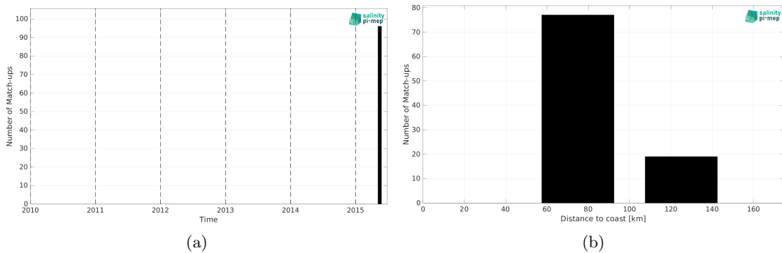
Figure 1: Number of match-ups between TSG (SAMOS) and SMOS SSS L3 v2 - 9-Days (BEC) SSS as a function of time (a) and as function of the distance to coast (b) over the Ganga and Brahmaputra river plumes Pi-MEP region and for the full satellite product period.
