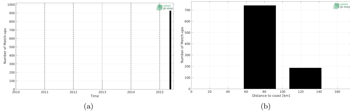
Figure 1: Number of match-ups between TSG (SAMOS) and SMOS SSS L3 v2 - 9-Days (BEC) SSS as a function of time (a) and as function of the distance to coast (b) over the Ganga and Brahmaputra river plumes Pi-MEP region and for the full satellite product period.
