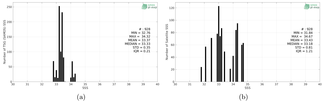
Figure 2: Histograms of SSS from TSG (SAMOS) (a) and SMOS SSS L3 v2 - 9-Days (BEC) (b) considering all match-up pairs per bins of 0.1 over the Ganga and Brahmaputra river plumes Pi-MEP region and for the full satellite product period.
