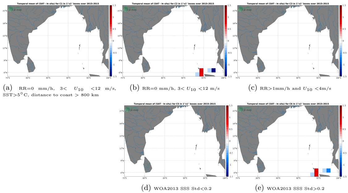
Figure 12: Temporal mean gridded over spatial boxes of size 1°x1° of \Delta SSS (SMOS SSS L3 v2 - 9-Days (BEC) - TSG (SAMOS)) for 5 different subdatasets corresponding to:RR=0 mm/h, 3 < U_{10} < 12 m/s, SST>5°C, distance to coast > 800 km (a), RR=0 mm/h, 3 < U_{10} < 12 m/s (b), RR>1mm/h and U_{10} < 4 m/s (c), WOA2013 SSS Std<0.2 (d), WOA2013 SSS Std>0.2 (e).
