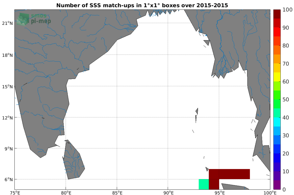
Figure 4: Number of SSS match-ups between TSG (SAMOS) SSS and the SMOS SSS L3 v2 - 9-Days (BEC) SSS product for the Ganga and Brahmaputra river plumes Pi-MEP region over 1^\circ \times 1^\circ boxes and for the full satellite product period.
