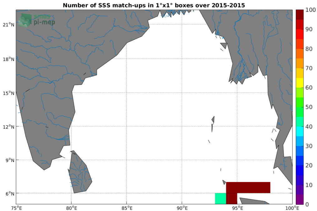
Figure 4: Number of SSS match-ups between TSG (SAMOS) SSS and the SMOS L3 v2 - 9-Days (BEC) SSS product for the Ganga and Brahmaputra river plumes Pi-MEP region over 1°x1° boxes and for the full satellite product period.
