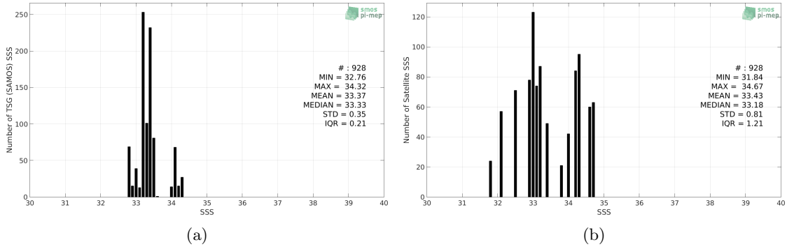
Figure 2: Histograms of SSS from TSG (SAMOS) (a) and SMOS L3 v2 - 9-Days (BEC) (b) considering all match-up pairs per bins of 0.1 over the Ganga and Brahmaputra river plumes Pi-MEP region and for the full satellite product period.
