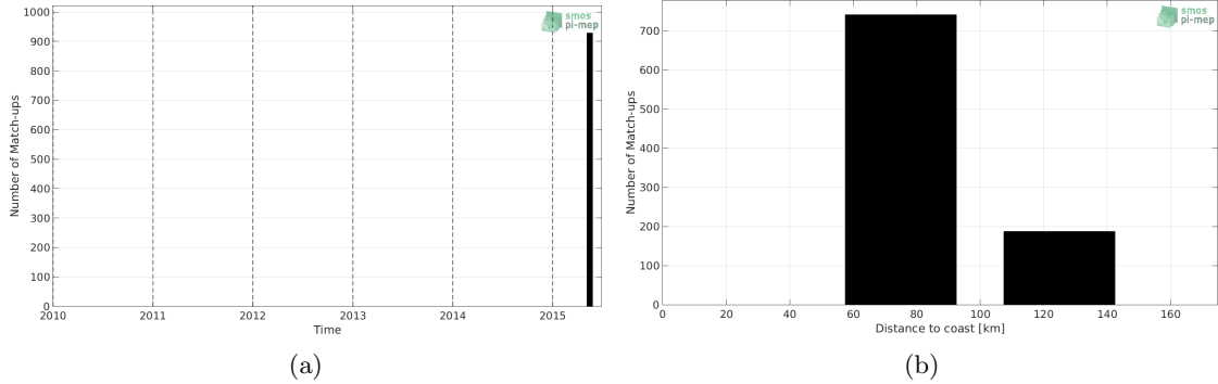
Figure 1: Number of match-ups between TSG (SAMOS) and SMOS L3 v2 - 9-Days (BEC) SSS as a function of time (a) and as function of the distance to coast (b) over the Ganga and Brahmaputra river plumes Pi-MEP region and for the full satellite product period.
