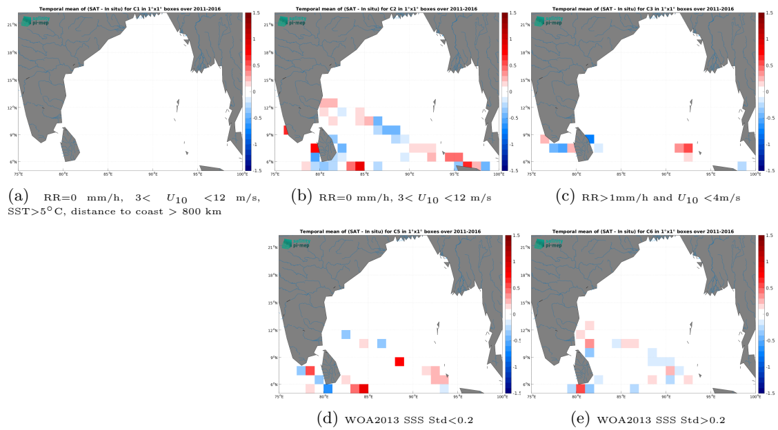
Figure 14: Temporal mean gridded over spatial boxes of size 1^\circ \times 1^\circ of \Delta SSS (SMOS SSS L3 v2 - 9-Days (BEC) - TSG (LEGOS-DM)) for 5 different subdatasets corresponding to: RR=0 mm/h, 3 < U_{10} < 12 m/s, SST > 5°C, distance to coast > 800 km (a), RR=0 mm/h, 3 < U_{10} < 12 m/s (b), RR > 1mm/h and U_{10} < 4 m/s (c), WOA2013 SSS Std < 0.2 (d), WOA2013 SSS Std > 0.2 (e).
