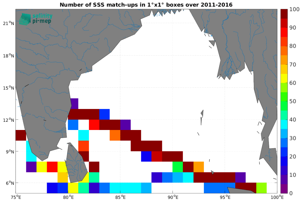
Figure 5: Number of SSS match-ups between TSG (LEGOS-DM) SSS and the SMOS SSS L3 v2 - 9-Days (BEC) SSS product for the Ganga and Brahmaputra river plumes Pi-MEP region over 1°×1° boxes and for the full satellite product period.
